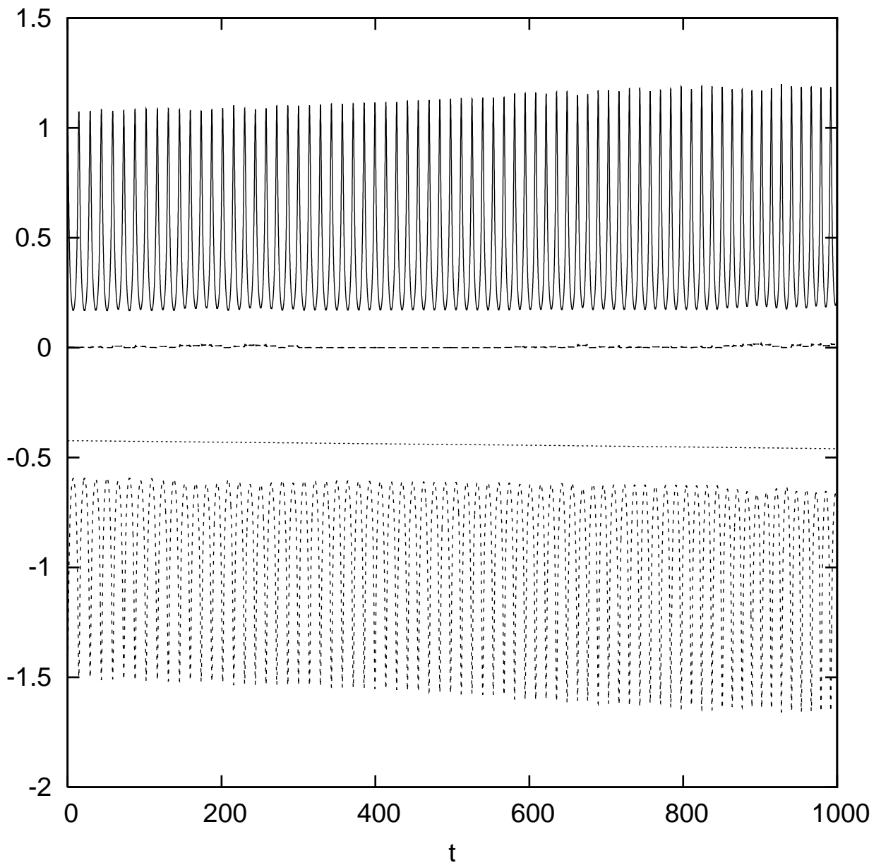
Orbiting Dumbbell Problem Elliptical Orbit -- Energy Quantities -- Tolerance=10(-6) Top to Bottom: KE_t, KE_r, E_tot, PE_g
