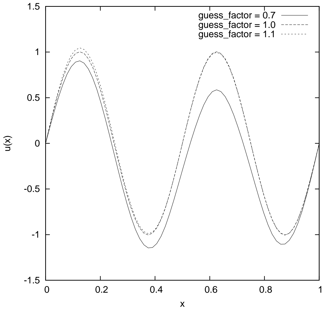
Three Distinct Solutions of Nonlinear BVP
