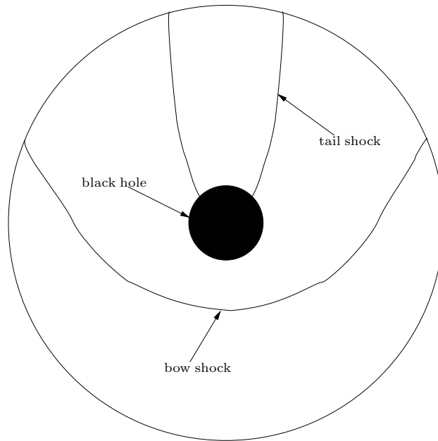
Figure A.10: The flow morphology for a typical simulation using the infinitely thin-disk approximation. We have clearly labelled the bow shock, black hole, and the tail shock in this diagram.
