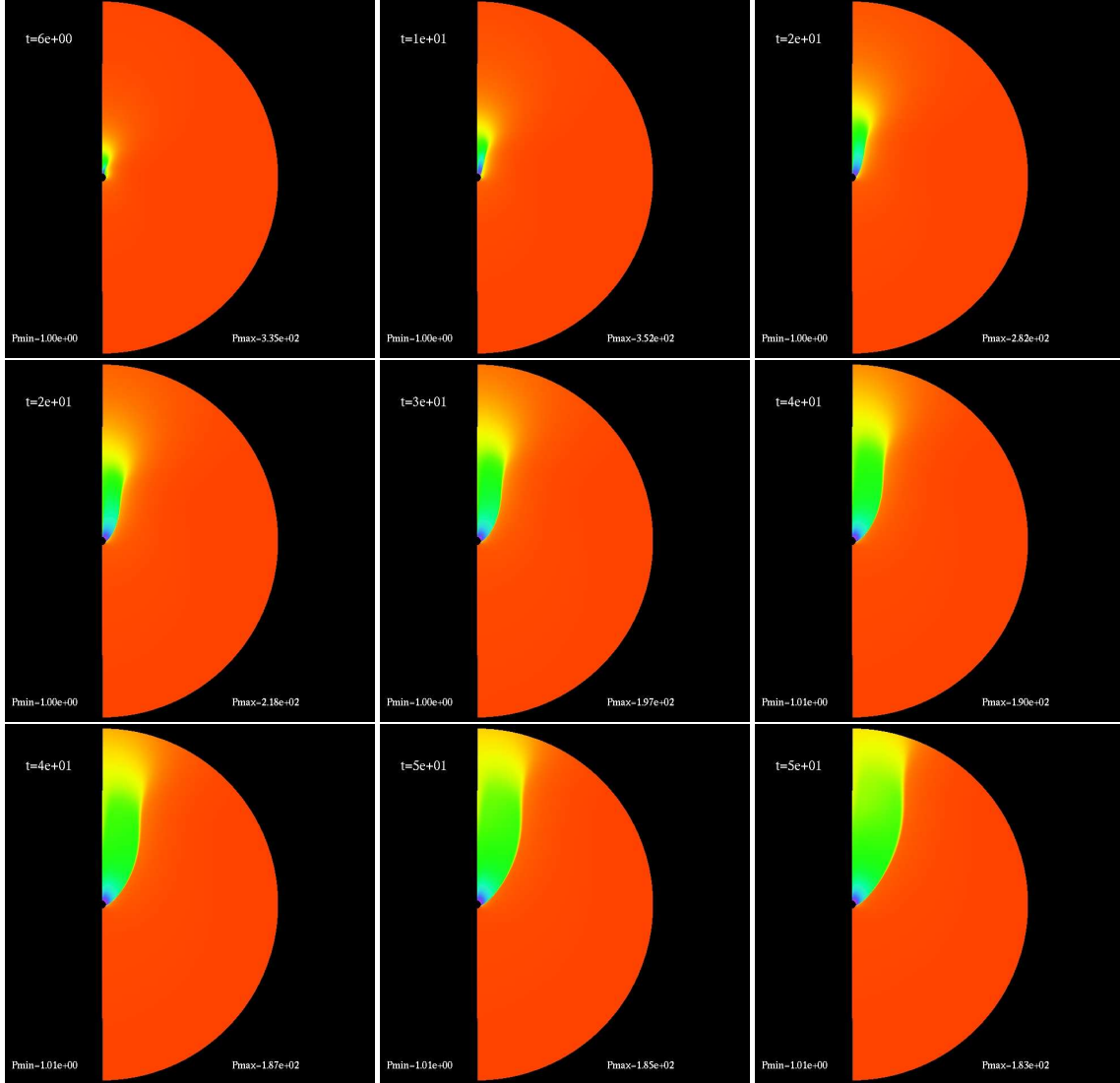
Figure A.7: Time evolution of P(t, r, \theta) for model U11 with a = 0.99 . As with other models the tail shock forms; however, here we see that the shock attaches to the black hole much closer to the upstream side.
