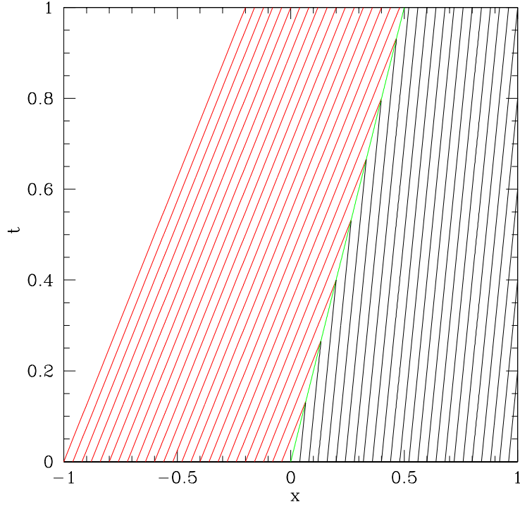
Figure 3.4: An example of a shock wave characteristic diagram for Burger's equation \partial_t q + \partial_x(q^2/2) = 0 , with initial data q(x, 0) = 0.8 if x < 0 ; q(x, 0) = 0.2 , if x \geq 0 . In this case the shock wave moves with speed, s , determined by the Rankine–Hugoniot jump conditions. For the Burger's equation we have, s = \frac{f(q_R) - f(q_L)}{q_R - q_L} = 0.5 , which is evident since the characteristic lines converge on the t = x/s line (green).
