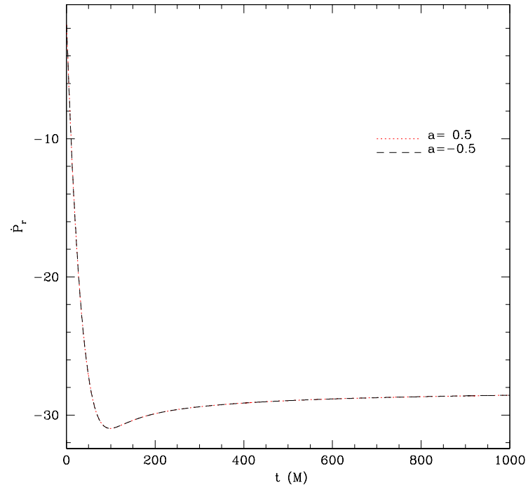
Figure 5.32: Ultrarelativistic radial momentum accretion rates for model U13 with a = \pm 0.5 . Just like the energy accretion seen in Fig. 5.30 we see that the accretion rates are identical.
