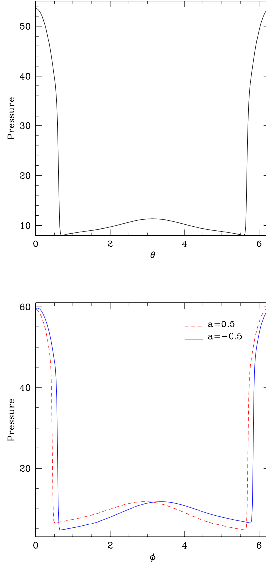
Figure 5.18: Ultrarelativistic pressure profile for the thin disk approximation for model U11 for r_{\text{max}} = 1000 . This cut is taken at the Schwarzschild radius. The a = 0 simulation at time t = 1000M (top) shows symmetry around the black hole while the a = 0.5 and a = -0.5 simulations at time t = 1000M (bottom) shows a deviation from the symmetry due to the rotation. The regions close to \phi = 0 and \phi = 2\pi are downstream of the black hole. The a = 0 simulation shows that there is only a small pressure difference between the upstream and downstream sides of the black hole. The rotating black hole exhibits a larger pressure in the downstream region, while the pressure in the upstream part of the domain, \pi/2 < \phi < 3\pi/2 , is similar to the a = 0 model.
