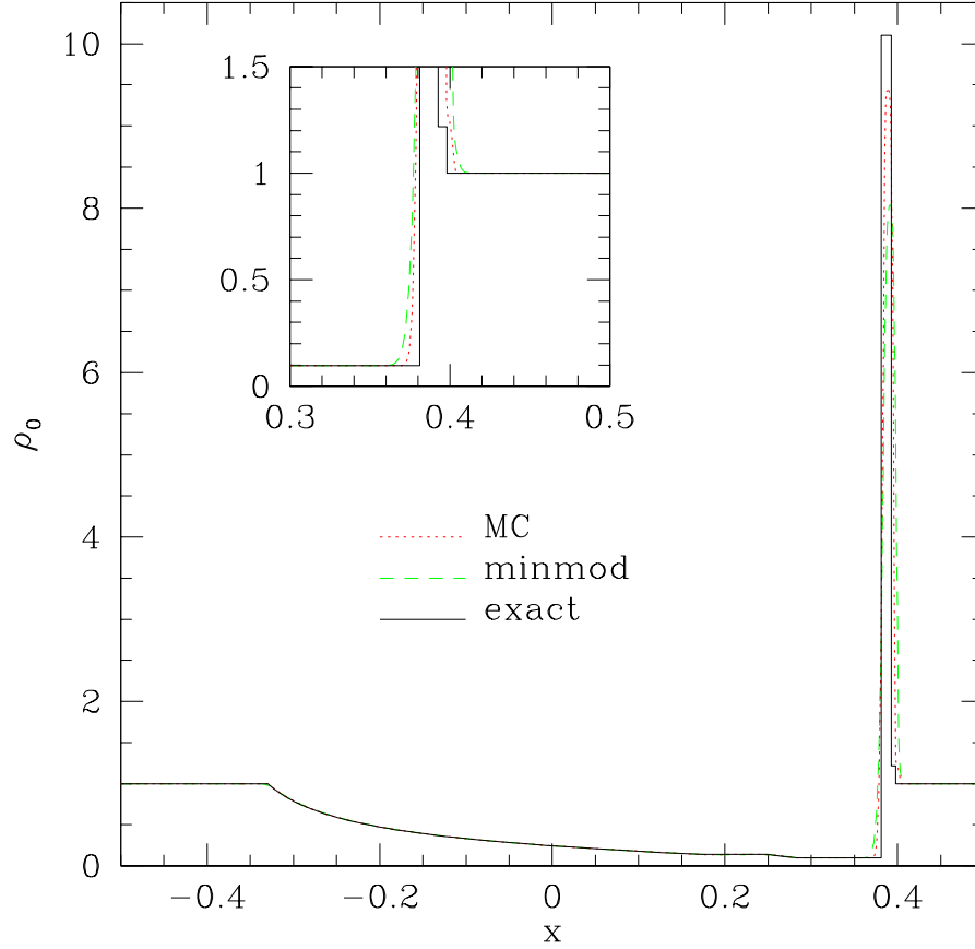
Figure 4.7: The one dimensional strong blast wave at a higher resolution. We use the domain -0.5 \leq x \leq 0.5 , with a resolution N_x = 1601 . The dotted line represents the results while using of the MC limiter, while the dashed line is the result of using the minmod limiter. The exact solution is the solid line. The higher resolution test shows evidence that the MC limiter offers a better representation of shocks than the midmod limiter. Once again the density amplitude while using the MC limiter is closer to the exact solution [52], but also in the blown up region around x = 0.4 we see that the MC limiter begins to capture the contact discontinuity that the minmod limiter is too diffusive to capture.
