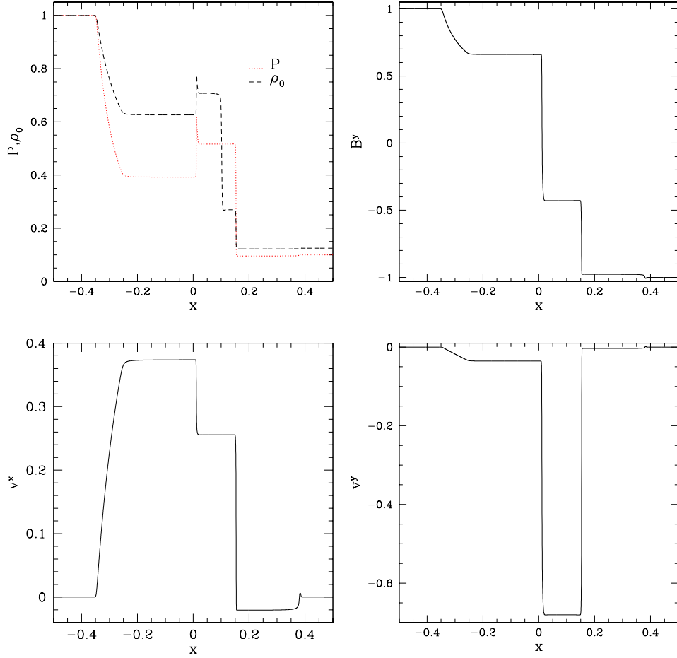
Figure 4.2: The Balsara blast wave test as designed by Balsara [47]. Plotted are the pressure, density (top), v^x (bottom left), B^y (top right), and v^y (bottom right). The interesting parts of this plot include the existence of a shock wave, a rarefaction wave, Alfvén wave and a contact discontinuity where the pressure is constant but the density exhibits a sharp discontinuity. This is a result of using the HLL solver with c_h = 1.0 , and N_x = 6400 . The solution shown here is at t = 0.4 , initial data are in the second two rows of table 4.1.
