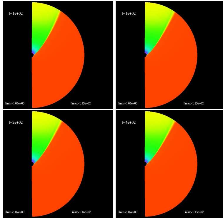
Figure A.6: Longer time evolution for model U7 with a = 0.5 .
