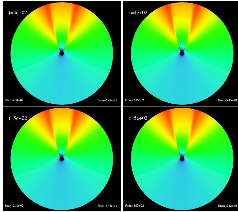
Figure A.12: Time evolution of the thin-disk accretion of P(t, r, \phi) for model U12 with a = 0 . We plot the pressure profile here; other scalar fields look similar. The last several frames shows that the evolution has become steady state.
