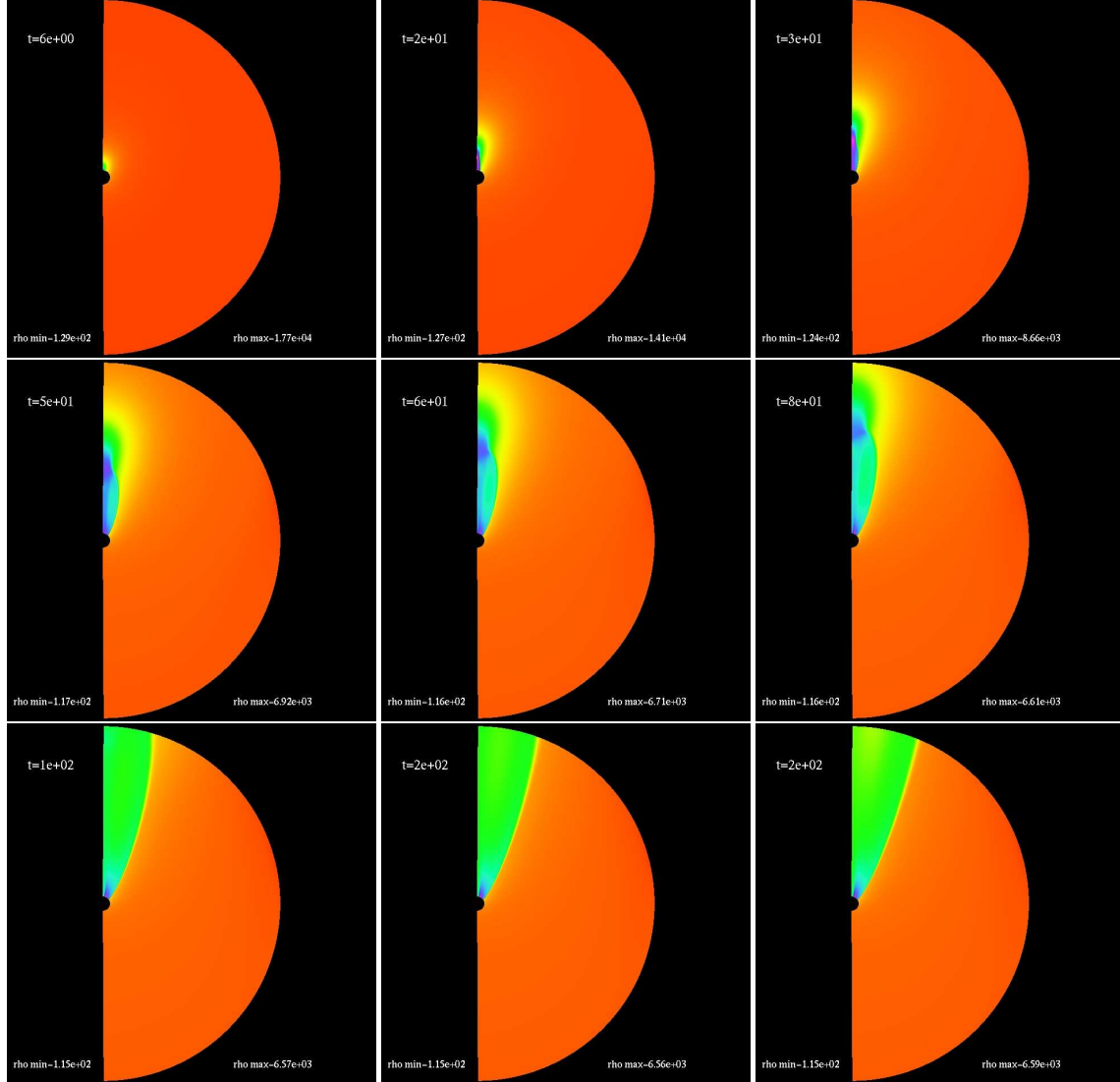
Figure A.17: Time evolution of the axisymmetric of \rho_0(t, r, \theta) accretion for model M1 with a = 0 . We plot the log of the density profile here. The last several frames shows that the density evolution has reached a steady state.
