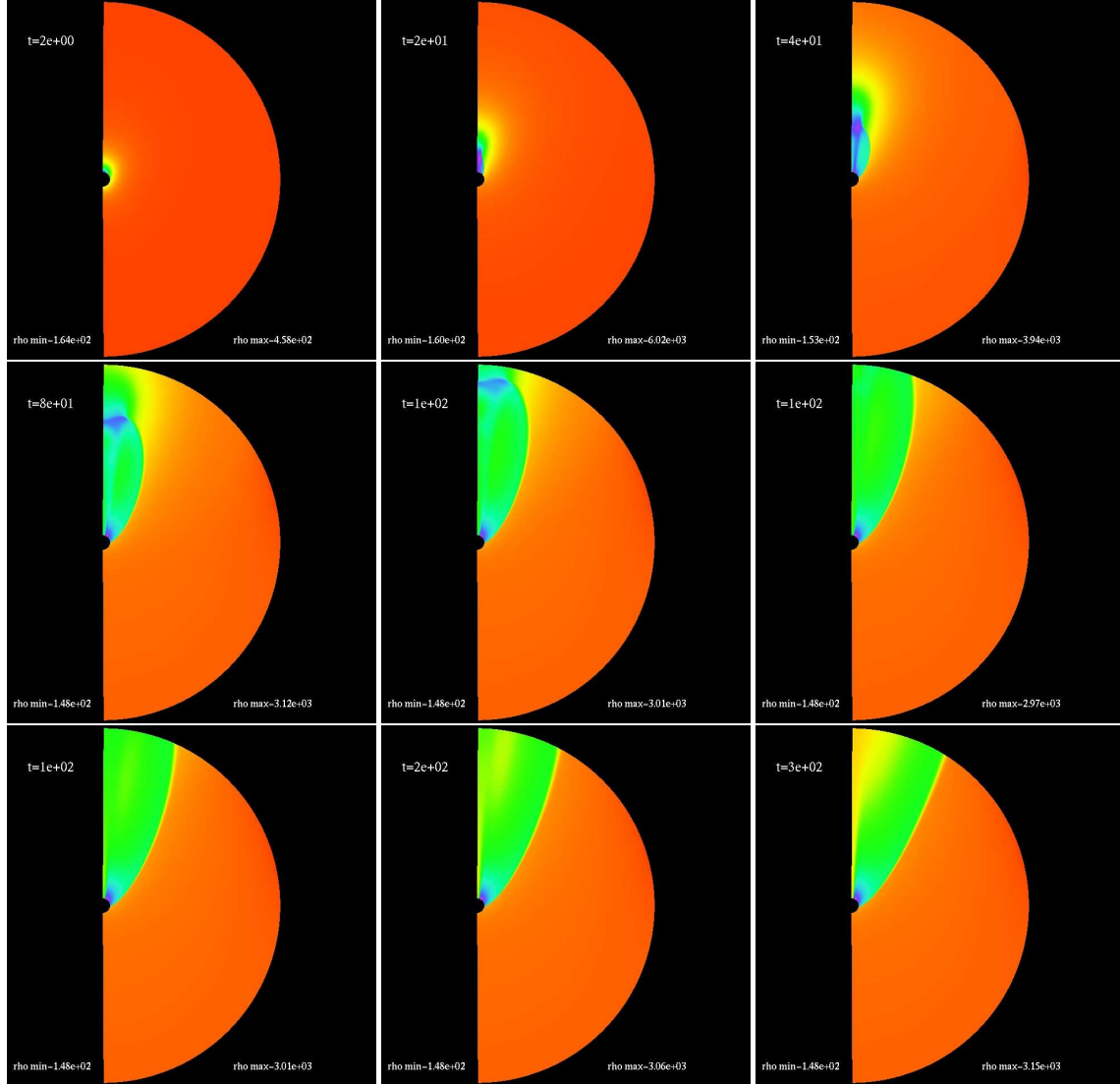
Figure A.18: Time evolution of the axisymmetric accretion of \rho_0(t, r, \theta) for model M2 with a = 0 . We plot the log of the rest mass density profile here. The last several frames shows that the rest mass density evolution has not reached a steady state in the time presented.
