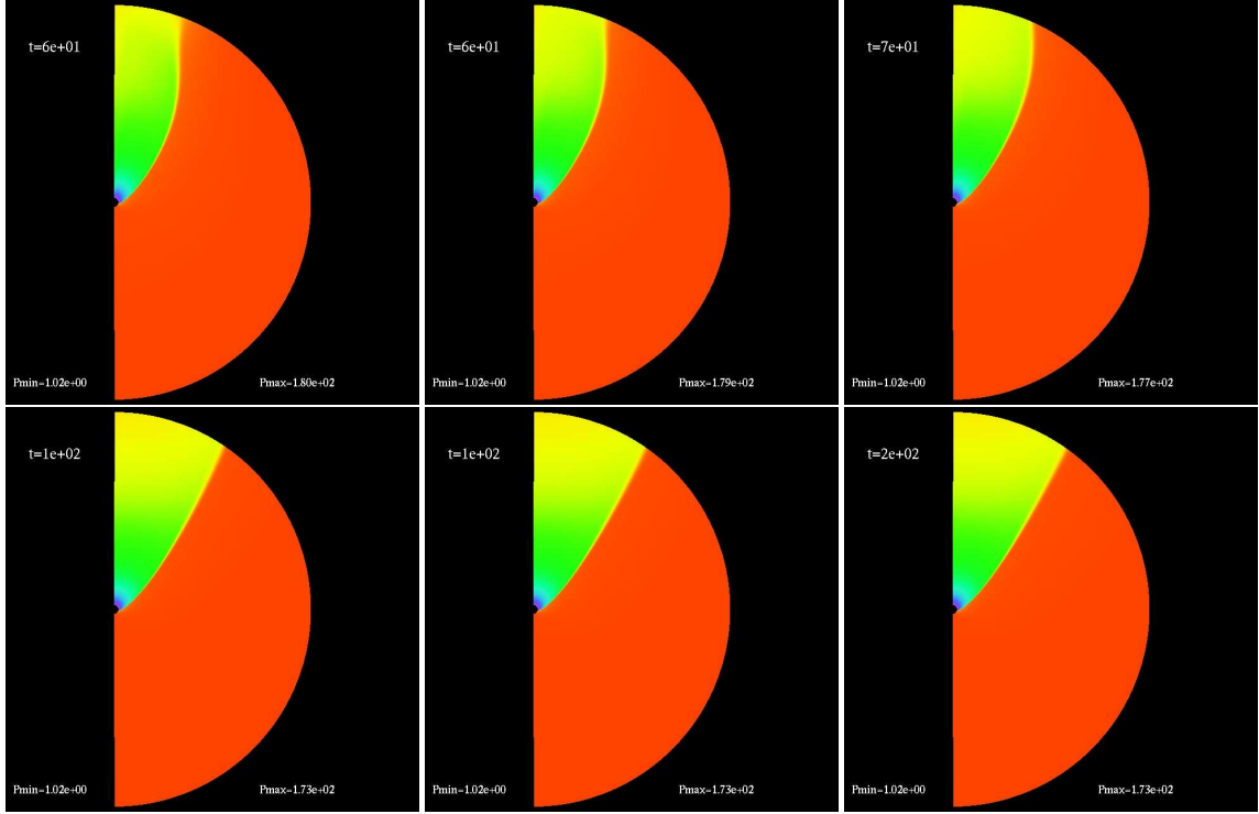
Figure A.8: Longer time evolution of P(t, r, \theta) for model U11 with a = 0.99 . The flow reaches a steady state.
