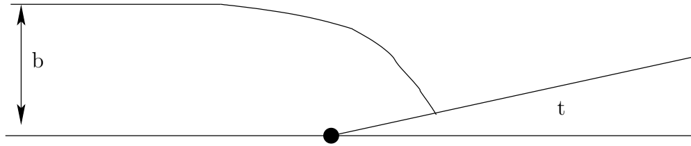
Figure 1.2: The original Bondi–Hoyle geometric setup. This setup is identical to the Hoyle–Lyttleton approach with the exception that the accretion column, the region labelled ‘t’, that forms behind the point mass is also considered. By including the accretion column the Hoyle–Lyttleton accretion rate was found to reduce by half.
