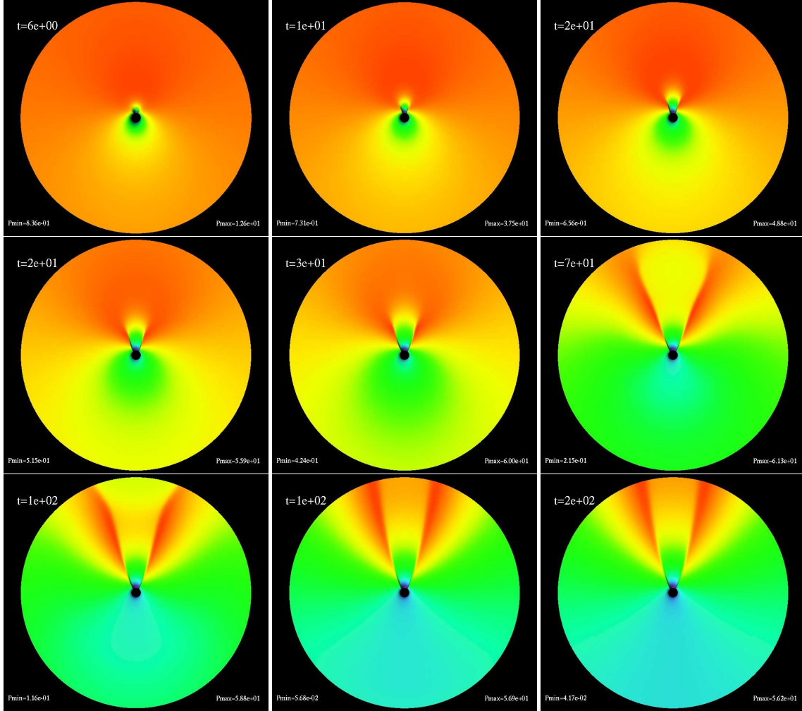
Figure A.11: Time evolution of the infinitely thin-disk accretion of P(t, r, \phi) for model U12 with a = 0 . We plot the logarithm of the pressure profile here; other scalar fields have a similar profile. The tail shock is clearly visible.
