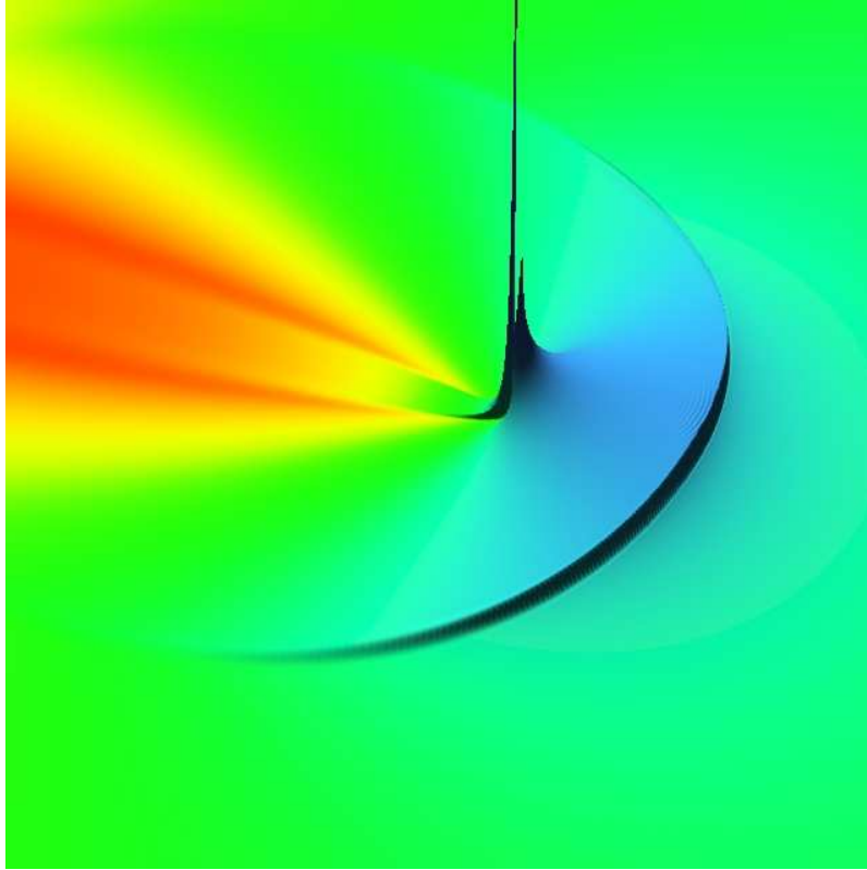
Figure A.16: A snapshot of the pressure for model U13 at time t = 500M . In this image the black hole is travelling diagonally across the page. This image clearly shows that the bow shock moving upstream is sharply defined even with a low resolution \Delta r = 0.25 .
