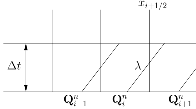
Figure 3.11: The CFL condition for a one dimensional cell. For the solution of the conservation equations (3.1) to be convergent we require that the time step, \Delta t , be small enough that the characteristics do not have enough time to interact with cells beyond the adjacent cell. This condition must be met for convergence to be possible; however, satisfying this condition alone does not guarantee convergence.
