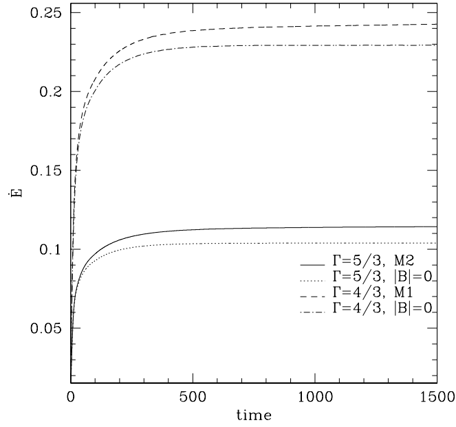
Figure 5.50: The relativistic Bondi-Hoyle energy accretion for models M1 and M2 with the corresponding simulations with no magnetic field present. The magnetic field energy accretion rate, \dot{E}_M (bottom), has not yet settled in the time shown here, but the total energy, \dot{E} (top), is clearly steady, which indicates that the hydrodynamic energy contribution in this simulation dominate the system. The trend shown in the total energy accretion rate is in agreement with the hydrodynamic systems studied in Font et al. [1]. The oscillations in the magnetic energy accretion rate decrease as a function of resolution.
