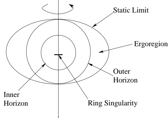
Figure 2.2: A Schematic for the Axisymmetric Spacetime.
