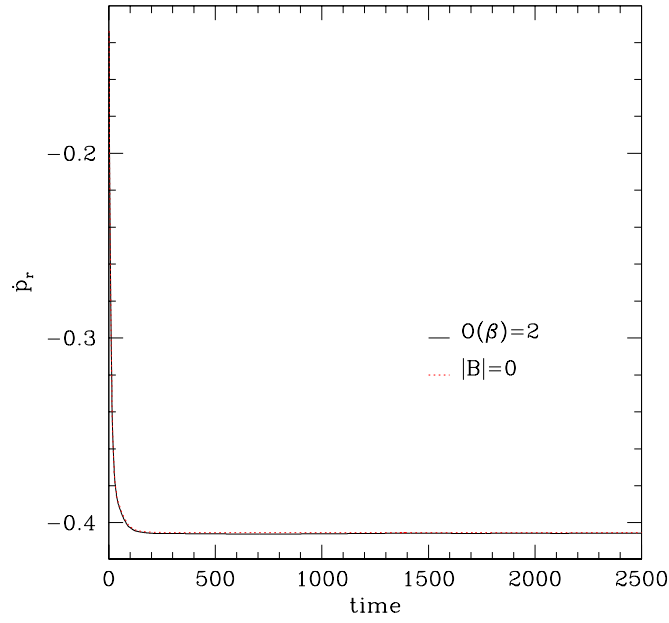
Figure 5.59: The relativistic Bondi–Hoyle accretion simulation for model M3 with a = 0.5 . The magnetic field has not settled in the time shown here, but the hydrodynamic variables are clearly steady. We present the radial momentum accretion rate with and without the presence of the magnetic field. It is evident that the magnetic field does not have a large impact on the momentum accretion rate.
