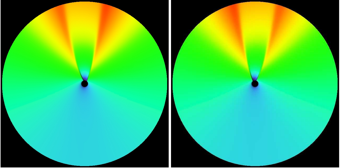
Figure 5.29: Ultrarelativistic accretion for model U13 with a = \pm 0.5 . For this simulation, r_{\text{max}} = 1000M , but we focus on the region 2 \leq r \leq 50 . This image was taken at time t = 500M and we present the logarithm of the pressure to emphasize the tail shock. We see that near the black hole the pressure profile wraps around the black hole; however, a few Schwarzschild radii away and the flow recovers a profile similar to that of the non-rotating black hole. We see that the flow morphology around an a = 0.5 black hole is a mirror image to the morphology around an a = -0.5 black hole. The similarity between rotating and counter-rotating black holes is emphasized in the accretion rate plots in Figs. 5.30 and 5.32
