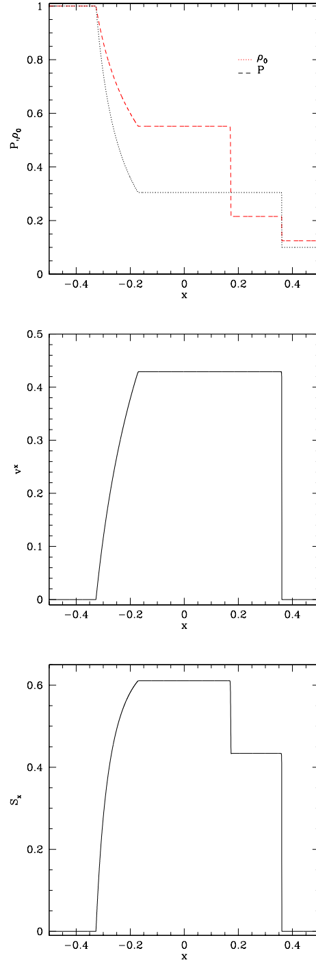
Figure 4.1: The Sod tube test [19]. Plotted are the pressure, density, v^x (middle), and S_x (bottom). The interesting parts of this plot include the existence of a rarefaction wave, a shock wave, and a contact discontinuity where the pressure is constant but the density exhibits a sharp discontinuity. This is a result of using the HLL solver with c_h = 1.0 , and N_x = 6400 . The solution shown here is at t = 0.4 , initial data are in the first two rows of table 4.1.
