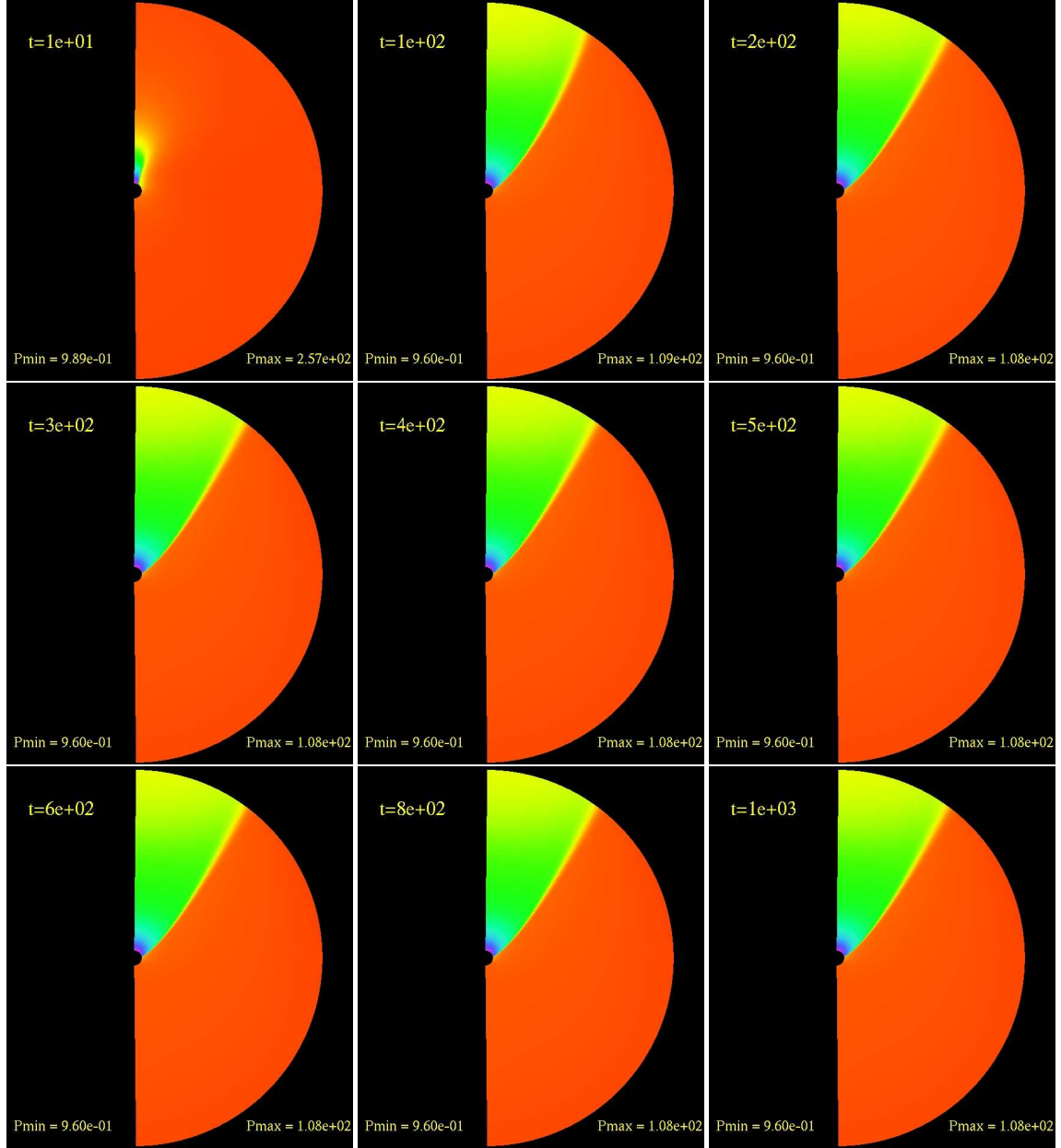
Figure A.4: Time evolution of P(t, r, \theta) for model U4 with a = 0 . We see the evolution of the ultrarelativistic fluid as it flows past the black hole. The formation of the a tail shock is evident in the first two frames. This shock begins to expand, but does not break contact with the black hole. The last several frames show that the fluid flow is steady.
