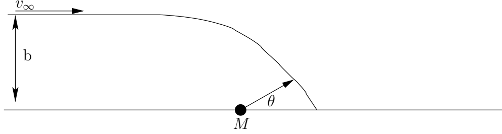
Figure 1.1: The original Hoyle–Lyttleton geometric setup. A particle with uniform asymptotic velocity v_\infty with an impact parameter b travels towards the massive body, M . As it passes the point mass the trajectory is altered, and if the particle is close enough to the point mass the particle will converge onto the x -axis, as shown by the solid black line.
