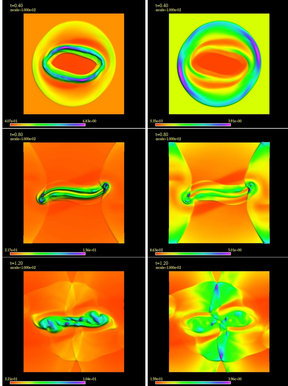
Figure 4.13: The results of the rigid rotor initial conditions with resolution 128 \times 128 , from top to bottom T = 0.4, 0.8, 1.2 . The left column shows the results for the baryon density \rho_0 , and the right column shows the results for the thermodynamic pressure P . The presence of a magnetic field is apparent in the first frame, where we see a flattened rotating fluid disk.
