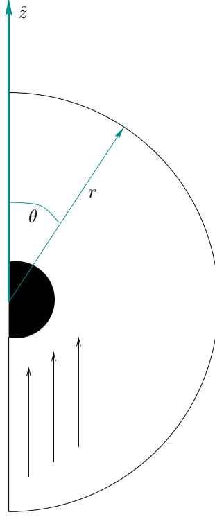
Figure A.1: The axisymmetric accretion setup. The flow enters from the domain boundary in the “upstream region” along \pi/2 \leq \theta \leq \pi and flows up past the black hole represented by the black semi-circle in the middle of the domain. The fluid then enters the downstream region and, unless flowing into the black hole will proceed to the downstream outer domain along 0 \leq \theta < \pi/2 where it flows out of the domain.
