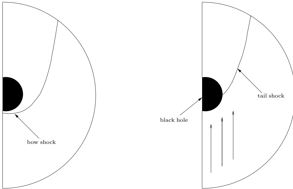
Figure A.2: A diagram containing the major features present in the following flow profiles. On the left we present the flow with a bow shock, while on the right we present a flow with a tail shock.
