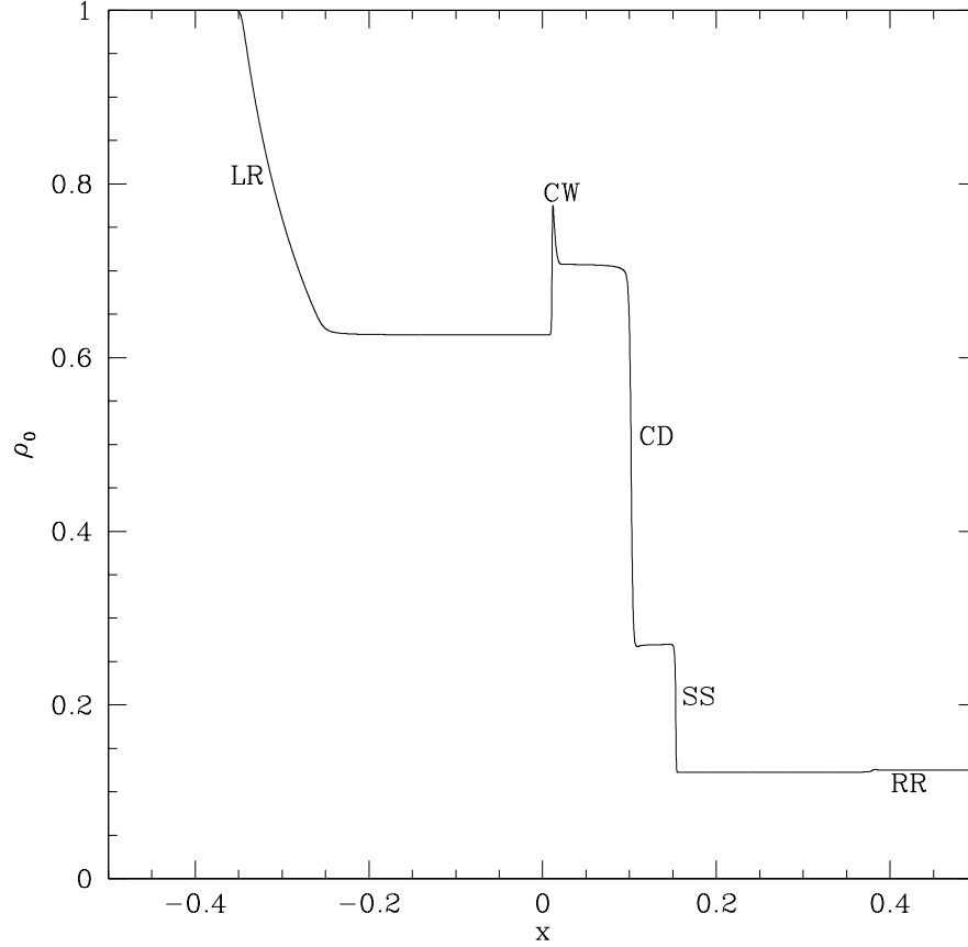
Figure 4.3: The density plot of the relativistic Balsara blast wave test [47]. When compared to Fig. 4.2, we label the different wave forms that develop. It is noted that some of the wave combinations are unique to magnetohydrodynamic systems. The labels are as follows: LR denotes a left moving rarefaction wave; and CW denotes a compound wave. The compound wave is unique to MHD systems and consists of an over-compressive shock, and a rarefaction wave. CD denotes a contact discontinuity, which is easily recognized by noticing that the pressure is constant across this discontinuity as seen in Fig. 4.2. SS denotes a slow shock and RR denotes a right moving rarefaction [150, 151].
