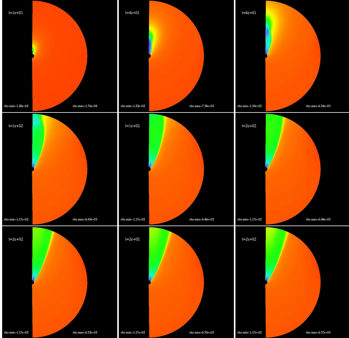
Figure A.19: Time evolution of the axisymmetric accretion of \rho_0(t, r, \theta) for model M3 with a = 0.5 . We plot the log of the density profile here. The last several frames shows that the density evolution has reached a steady state.
