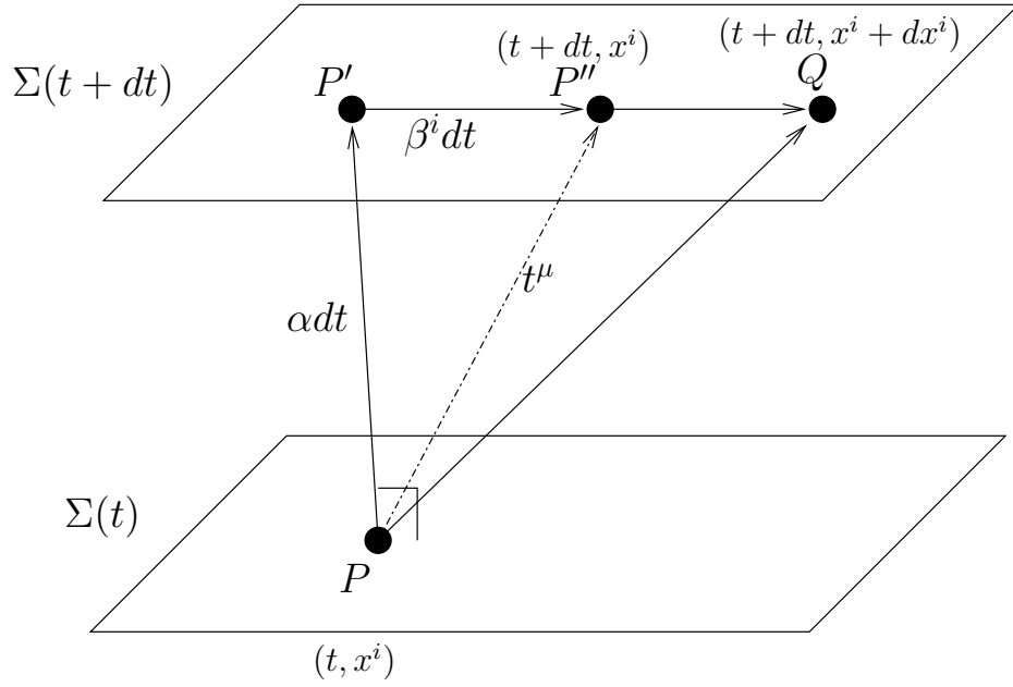
Figure 2.1: The 3+1 decomposition of relativistic spacetime. The spacetime is foliated into space-like hypersurfaces \Sigma(t) . Here we show two such slices at t and t+dt . The vector connecting the coordinate x^i on slice \Sigma(t) to x^i on slice \Sigma(t+dt) may be decomposed into a part orthogonal to the slice \alpha dt , and a part parallel to the slice \beta^i dt . To follow the dynamics of an event as it moves from event P at (t, x^i) to a new point Q at (t+dt, x^i + dx^i) requires that we also consider the spatial translation.
