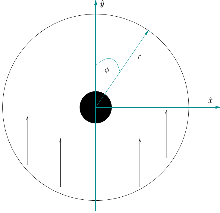
Figure A.9: The non-axisymmetric thin disk accretion setup. The material enters the domain along the \pi/2 \leq \phi \leq 3\pi/2 boundary, known as the upstream region. The fluid then flows “up” the page, past the black region in the diagram, denoting the black hole, to the downstream region where if it makes contact with the domain on -\pi/2 < \phi < \pi/2 the fluid leaves the domain of integration. We refer the reader to Fig. A.10 for a diagram of the shocks found in the flow morphology.
