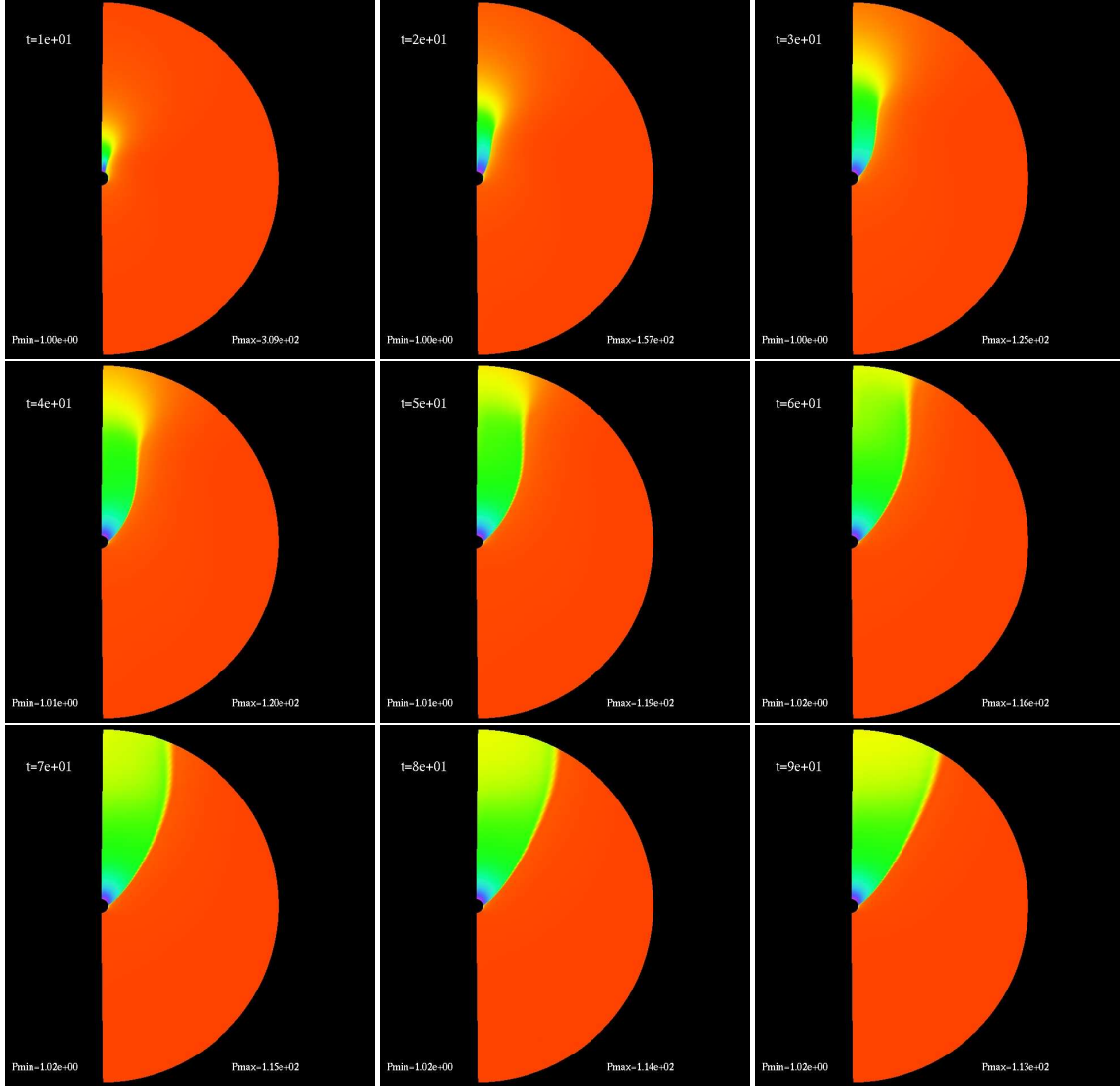
Figure A.5: Time evolution of P(t, r, \theta) for model U7 with a = 0.5 . We see the evolution of the ultrarelativistic fluid as it flows past the rotating black hole does not change morphology significantly when compared to the a = 0 black hole. Once again we have a tail shock and a steady flow.
