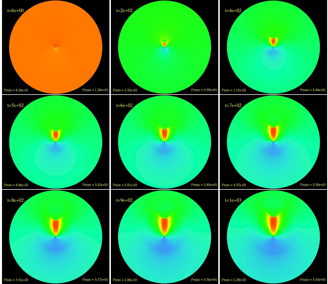
Figure A.14: Time evolution of the thin-disk accretion of P(t, r, \phi) for model U12 with r_{\max} = 1000 and a = 0 . We plot the logarithm of the pressure profile here, other scalar fields have a similar profile. The tail shock is clearly visible.
