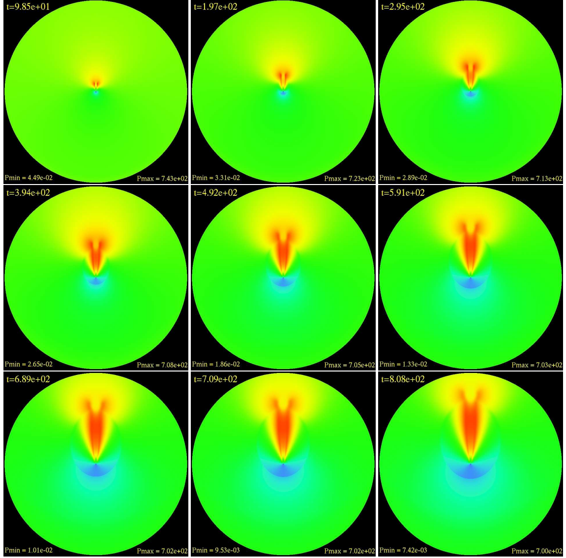
Figure A.15: Time evolution of the thin-disk accretion of P(t, r, \phi) for model U13 with r_{\max} = 1000 and a = 0 . When the flow is faster the width of the tail shock decreases.
