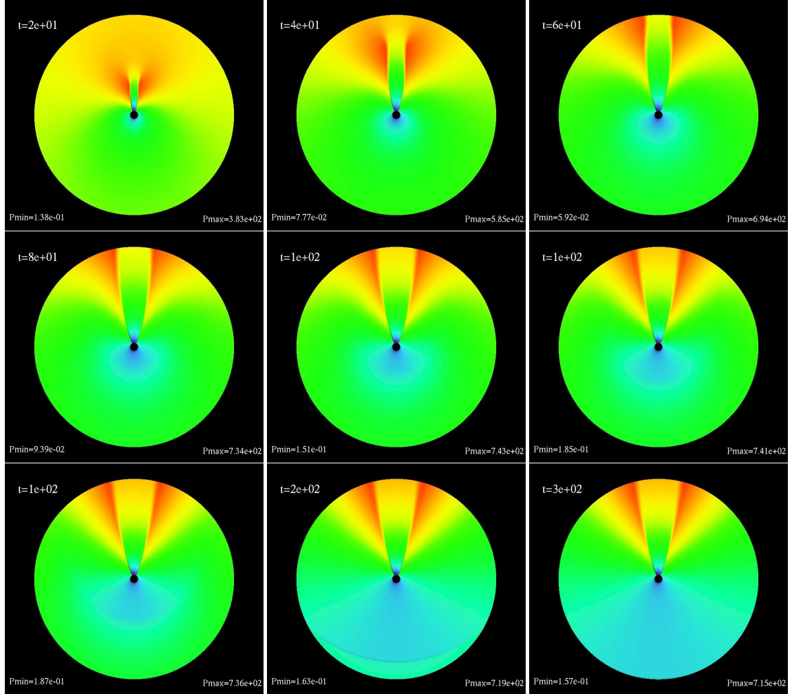
Figure A.13: Time evolution of the thin-disk accretion if P(t, r, \phi) for model U13 with a = 0 . When the flow is faster the width of the tail shock decreases. Notice the wave impinging on the upstream boundary in the second last frame. When this makes contact with the boundary we expect an amplification of the boundary effects to enter the simulation.
