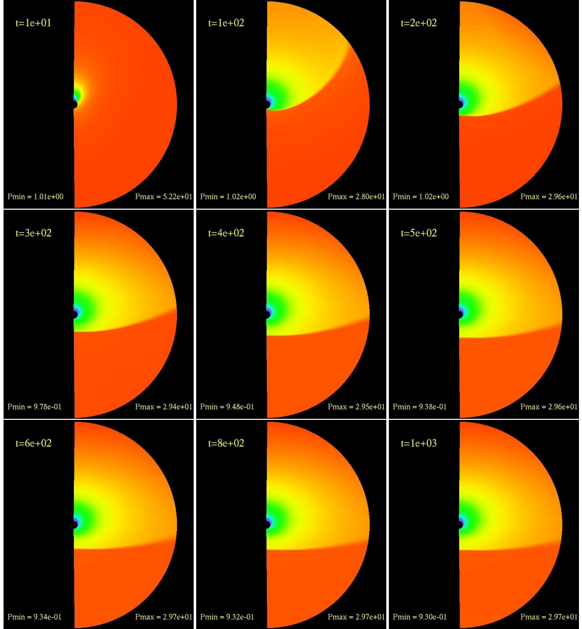
Figure A.3: Time evolution of P(t, r, \theta) for model U2 with a = 0 . We see the evolution of the ultrarelativistic fluid as it flows past the black hole. The formation of the a tail shock is evident in the first two frames. This shock expands quickly and eventually detaches from the black hole by the 4th frame. In the last two frames we see the detached shock flow upstream.
