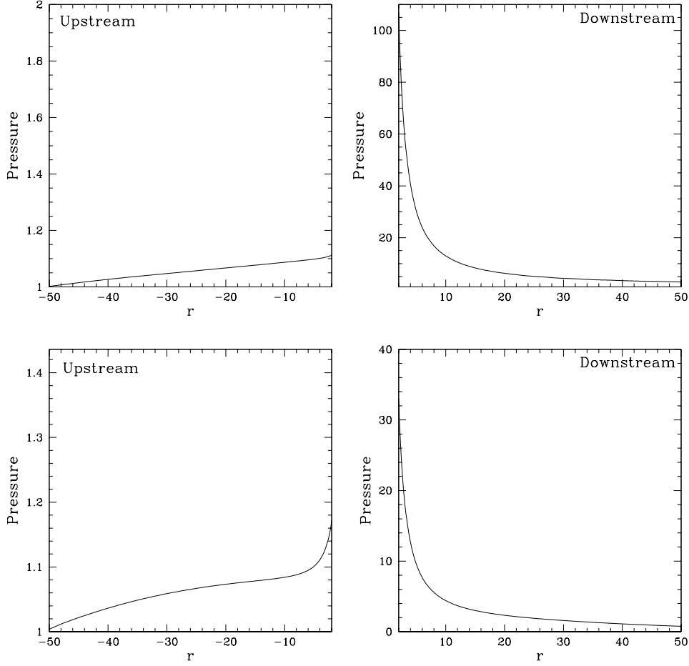
Figure 5.2: Ultrarelativistic pressure profile in the upstream, \theta = \pi/2 , (left column) and downstream, \theta = 0 , (right column) regions for model U3 (top) and U4 (bottom). We see that the pressure in the upstream region of the black hole is small by comparison to the pressure in the wake in the downstream region. The image on the left is magnified to show that there is a slight increase in pressure as the fluid reaches the black hole. As the asymptotic velocity of the black hole increases the upstream pressure deviates less from the pressure defined at the boundaries. Since the upstream pressure profile does not smoothly agree with the upstream boundary condition, a larger domain was required for simulations of slower black holes.
