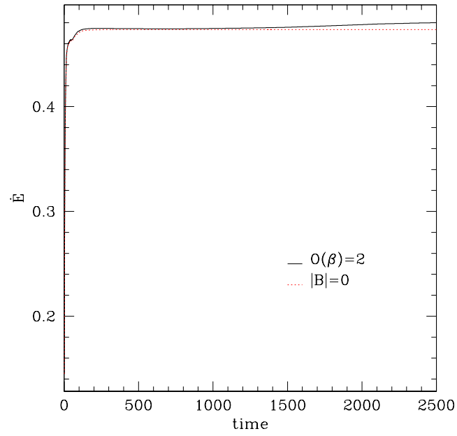
Figure 5.58: The relativistic Bondi–Hoyle energy accretion for model M3. The magnetic field has not settled in the time shown here, but the total energy is clearly steady, which indicates that the hydrodynamic energy contribution in this simulation dominates the system.
