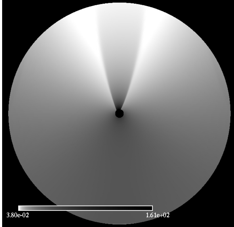
Figure 5.28: Ultrarelativistic accretion for model U13 with a = 0.5 . For this simulation, r_{\text{max}} = 50 . This image was taken at time t = 500M before the boundary effects were found to effect the accretion process. The morphology of the pressure flow rotates around the black hole. The rotational effects of the black hole were localized to a few a few Schwarzschild radii. Beyond that, the flow morphology was found to be similar to that of accretion onto a spherically symmetric black hole. The region of contact between the tail shock and the black hole decreases as a function of the asymptotic velocity; however, none of the parameters investigated exhibited a disconnection between the tail shock and the black hole. These results agrees with the findings presented in FI99.
