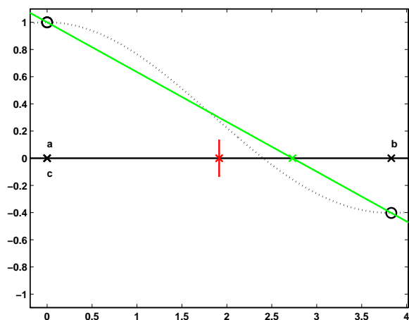
Figure 4.3. Initially, choose secant or bisection.
