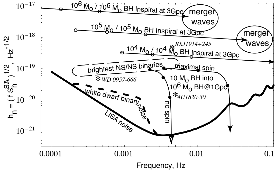
Figure 9.6: Projected noise curve h_n(f) for LISA, together with a number of promising sources of gravitational radiation in the low-frequency band (see Section 9.2.2). The thick line is LISA’s instrument noise; the thick-dashed curve is the noise curve incorporating the expected stochastic background of gravitational radiation from unresolved white-dwarf binaries. Wave strengths above these curves have sufficiently high signal-to-noise ratio that they should be detectable using optimal signal processing. [From Cutler and Thorne (2002).]
