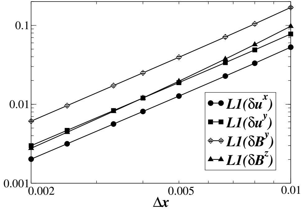
Figure 5.3: L1 norms of the errors in u^x , u^y , B^y and B^z for the nonlinear Alfvén wave test at t = t_{\text{final}} = 2.0 . This log-log plot shows that the L1 norms of the errors in u^x , u^y and B^y are proportional to (\Delta x)^2 , and are thus second-order convergent. The error in B^z goes as a slightly higher power of \Delta x . [From Duez et al. 2005b.]
