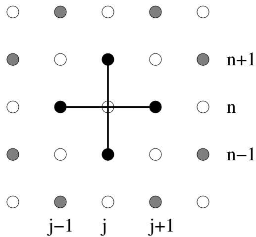
Figure 6.7: Finite difference stencil for the leap-frog scheme.
