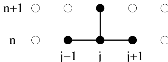
Figure 6.5: The finite-differencing stencil for the “forward-time centered-space” (FTCS) differencing scheme.
