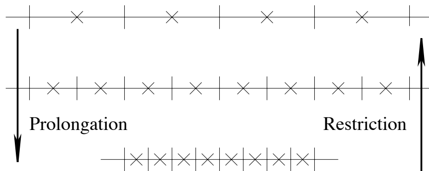
Figure 6.4: An illustration of a multigrid method.
