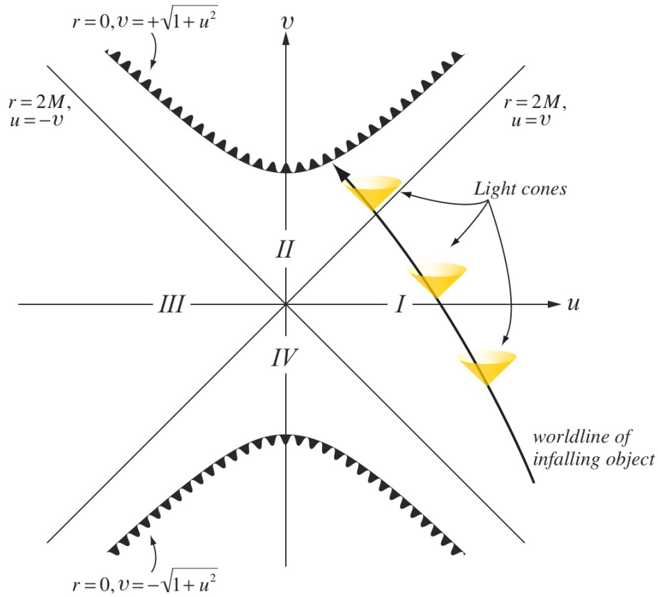
Figure 1.1: A Kruskal-Szekeres diagram. [After Shapiro and Teukolsky (1983).]
