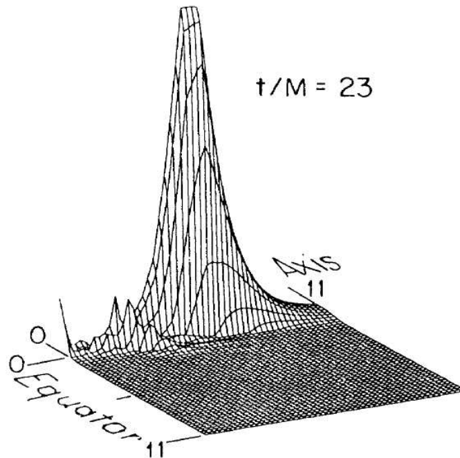
Figure 10.3: Profile of I in a meridional plane for the collapse shown in the right panels of Figure 10.1. For the case shown here employing 32 angular zones to cover one hemisphere, the peak value of I is 24/M^4 and occurs on the axis just outside the matter. [From Shapiro and Teukolsky (1991b).]
