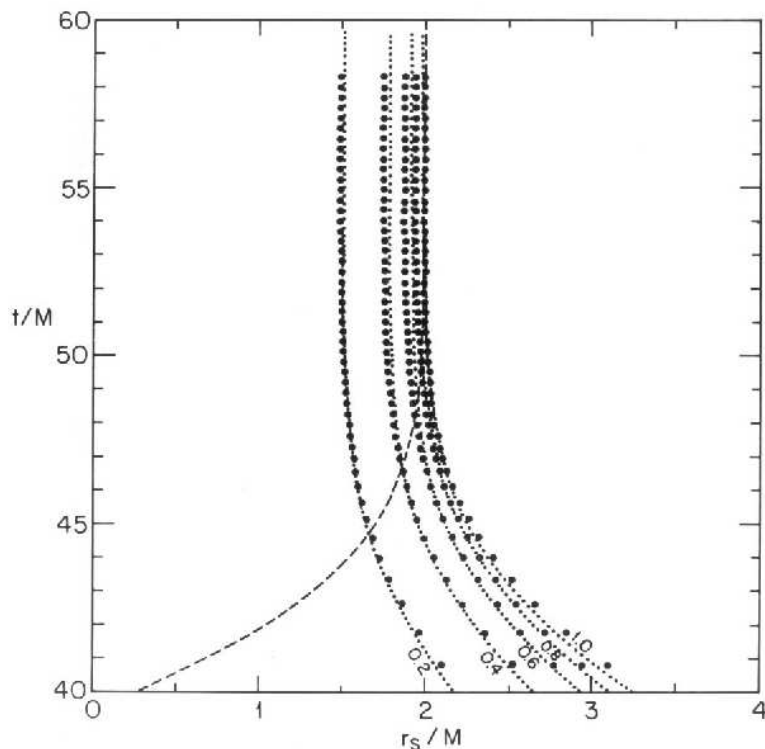
Figure 8.11: Spacetime diagram at late times for Oppenheimer-Snyder collapse in polar slicing from R = 10M . The labelling is the same as in Figure (8.10). No trapped surface forms in this slicing. [From Shapiro and Teukolsky (1986)].
