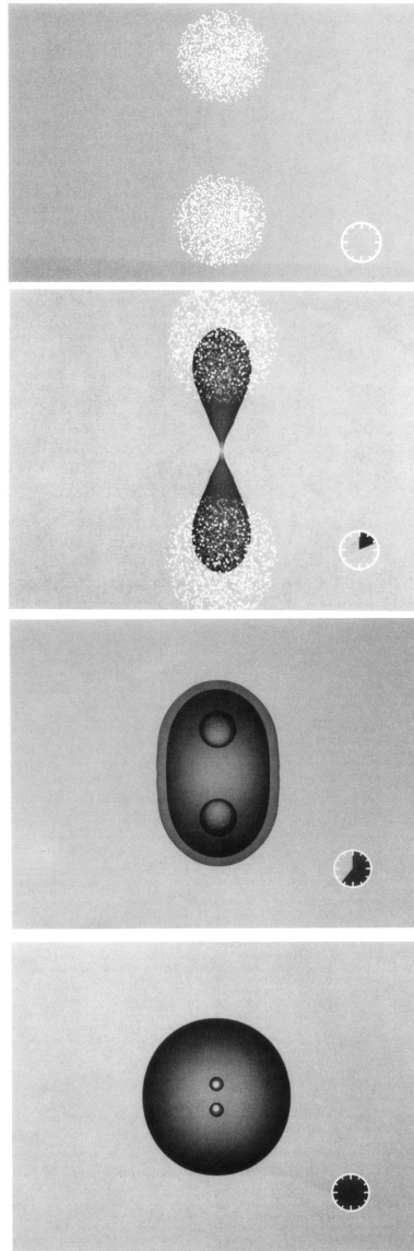
Figure 10.4: Spatial snapshots of the head-on collision of boosted clusters. (a) Initial data. Each sphere has an initial radius a/M = 0.8 , an inward boost velocity v = 0.15 , and their centers are at z_0/M = \pm 1.4 . Sample particles from the collisionless matter distribution are represented by white dots. A clock displaying the elapsed fraction of the total evolution time appears in the corner. (b) Horizon coalescence. At time t/M = 2.18 the two event horizons coalesce (shaded hour glass). The cluster's centers are at z/M = \pm 1.07 . The scale of the image has been enlarged by about a factor of 2 over (a). (c) Appearance of apparent horizons. At time t/M \approx 6.5 , the common apparent horizon appears, well inside the event horizon. At time t/M \approx 7.1 (shown here) the disjoint apparent horizons appear. The outer shaded region denotes the event horizon, the darker shaded region just inside is the common apparent horizon, and the two darkest regions are the disjoint apparent horizons. (d) Final state. By time t/M \approx 11.7 shown here, the event and common apparent horizons have settled down to a quasistationary state and coincide. [From Hughes et al. (1994).]
