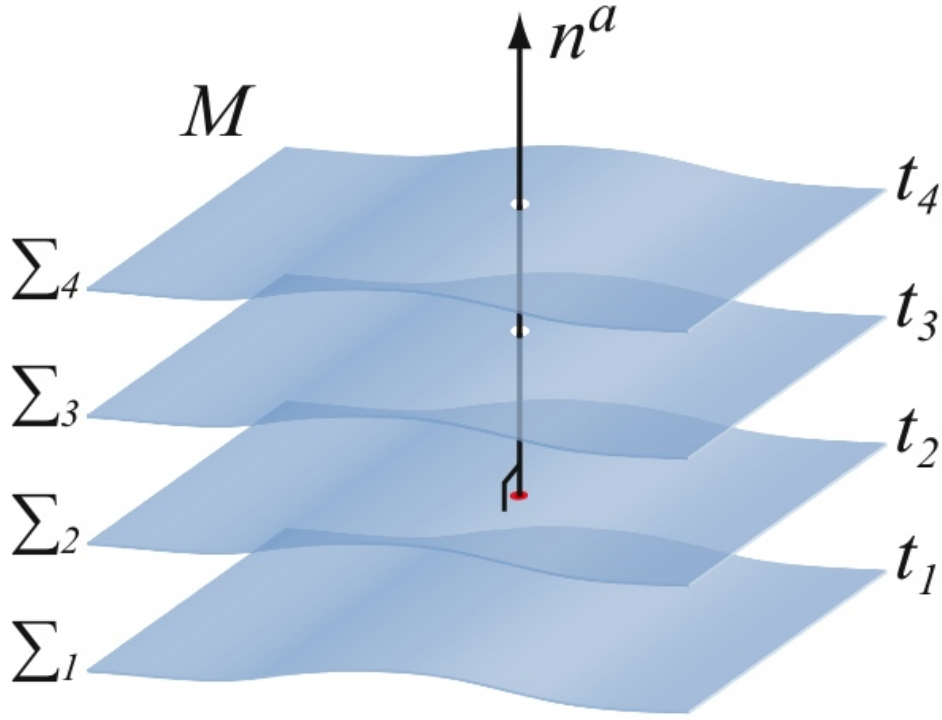
Figure 2.1: A foliation of the spacetime M . The hypersurfaces \Sigma are level surfaces of the coordinate time t , \Omega_a = \nabla_a t . The normal vector n^a is orthogonal to these t = \text{constant} spatial hypersurfaces.
