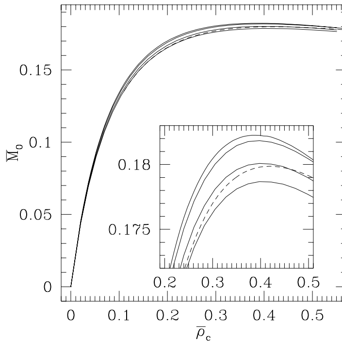
Figure 15.2: [CAMBRIDGE: replace \bar{\rho}_c with \bar{\rho}_c^* on x -axis.] Rest mass \bar{M}_0 versus central density \bar{\rho}_c^* along sequences of equal-mass, corotational binary companions obeying an n = 1 polytropic EOS. Successive curves are for binary separations ranging from s = 0.3 (bottom solid line), through 0.2 and 0.1, and extending to 0.0 (top line). The dashed line is the Oppenheimer-Volkoff limiting curve for isolated static stars ( s = 1 ). Due to finite difference errors, the numerical values systematically underestimate the mass, hence some of the curves creep below the Oppenheimer-Volkoff curve. The insert is a blow-up of the region around the maximum masses. [From Baumgarte et al. (1997).]
