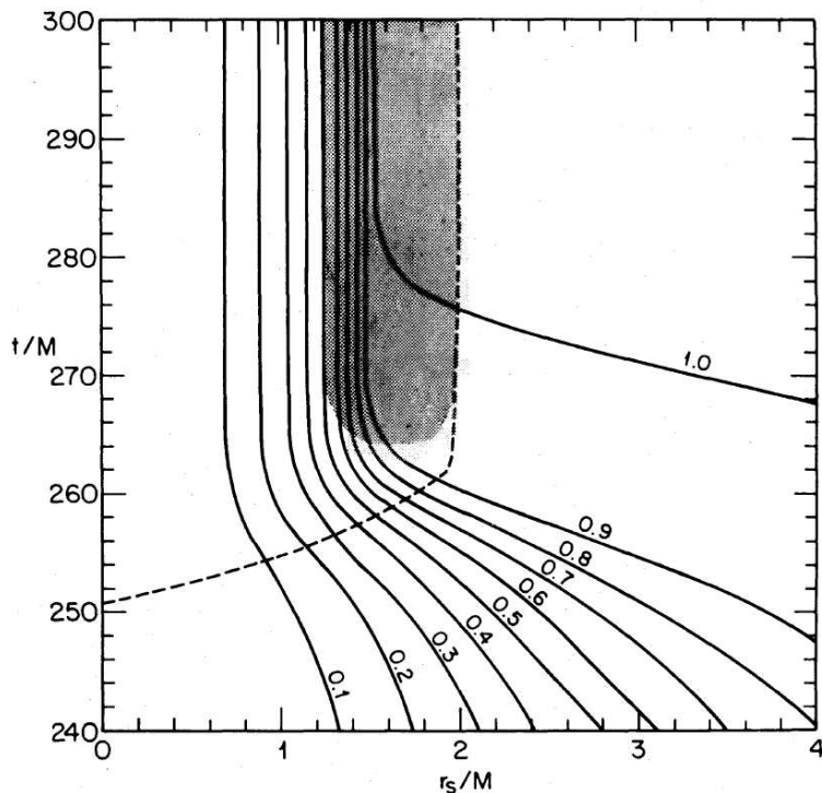
Figure 8.13: Spacetime diagram in maximal slicing for the Maxwell-Boltzmann cluster depicted in Figure (8.12). The solid lines are worldlines of fictitious Lagrangian matter tracers labelled by the fixed interior rest-mass fraction. The dashed line is the event horizon. The shaded area is the region of trapped surfaces. The event and apparent horizons both numerically asymptote to r_s = 2M to high accuracy. [From Shapiro and Teukolsky (1986)].
