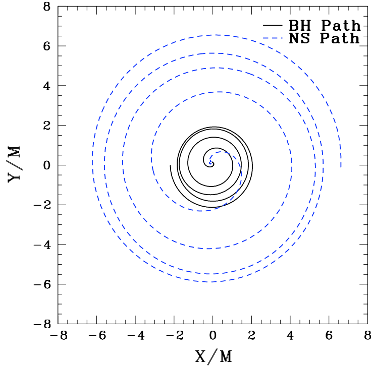
Figure 17.8: Trajectories of the black hole and neutron star coordinate centroids for the merger of an irrotational binary with mass ratio q = 3 (case A). The black hole (BH) centroid corresponds to the centroid of the apparent horizon, and the neutron star (NS) centroid is computed via the integral \tilde{X}_c^i \equiv (\int_V x^i \rho_* d^3x) / (\int_V \rho_* d^3x) , where V is the total simulation volume. [From Etienne et al. (2009).]
