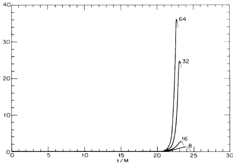
Figure 10.2: Growth of the Riemann invariant I (in units of M^{-4} ) versus time for the collapse shown in the right panels of Figure 10.1. The simulation was repeated with various angular grid resolutions. Each curve is labeled by the number of angular zones used to cover one hemisphere. Dots indicate where the singularity has caused the code to become inaccurate. [From Shapiro and Teukolsky (1991b).]
