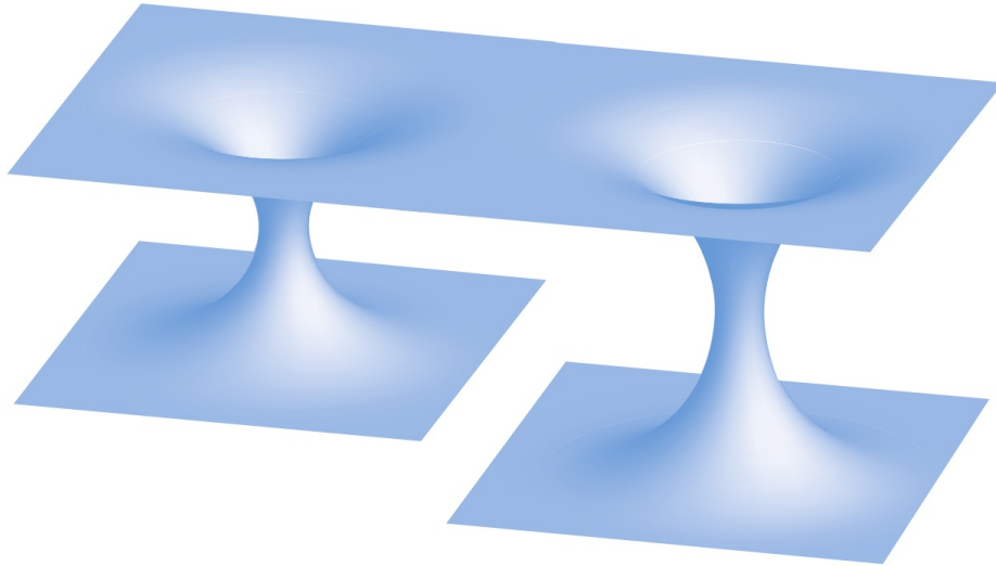
Figure 3.2: Schematic embedding diagram of the geometry described by metric (3.23) for two black holes at a moment of time symmetry. This is the three-sheeted topology, which does not satisfy an isometry across each throat.
