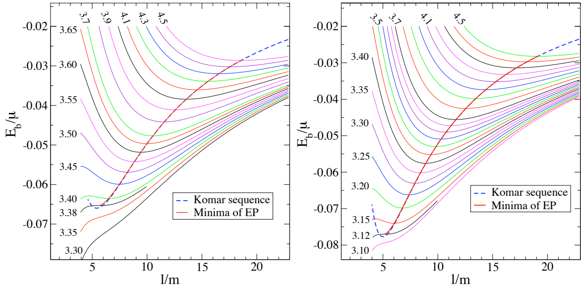
Figure 12.5: [CAMBRIDGE: replace m with M in label] The binding energy E_b versus separation l for corotational (left panel) and nonspinning (right panel) equal-mass binary black hole sequences constructed in the conformal thin-sandwich approach. The solid lines connecting the extrema of the curves of constant angular momentum, which are labeled by J/\mu M , represent sequences constructed with the effective potential method as in Figure 12.3; these lines terminate at the ISCO. The dashed lines represent sequences constructed from the mass criterion (12.108). These sequences agree extremely well up to very small separations, where the assumption of quasiequilibrium breaks down. [From Caudill et al. (2006).]
