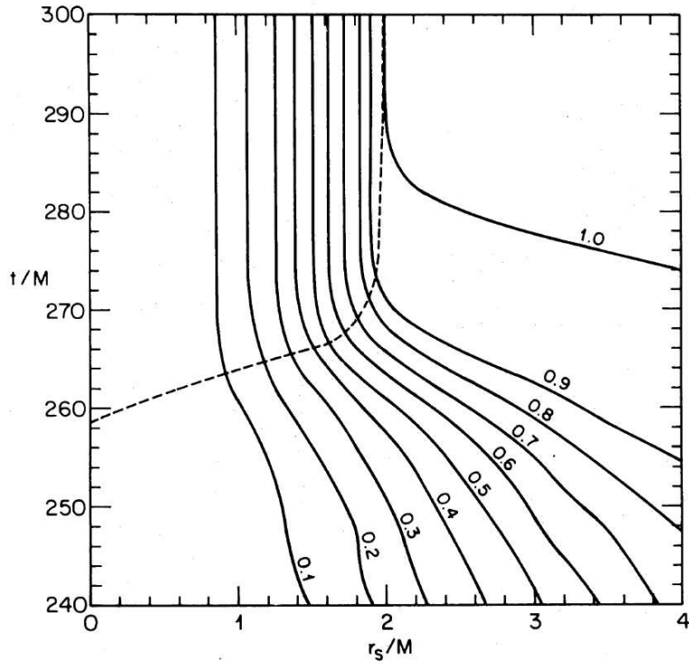
Figure 8.14: Spacetime diagram in polar slicing for the Maxwell-Boltzmann cluster depicted in Figures (8.12) and (8.13). Labelling is the same as in Figure (8.13). No trapped surface forms in polar slicing. The event horizon and matter surface both numerically asymptote to r_s = 2M to high accuracy. [From Shapiro and Teukolsky (1986)].
