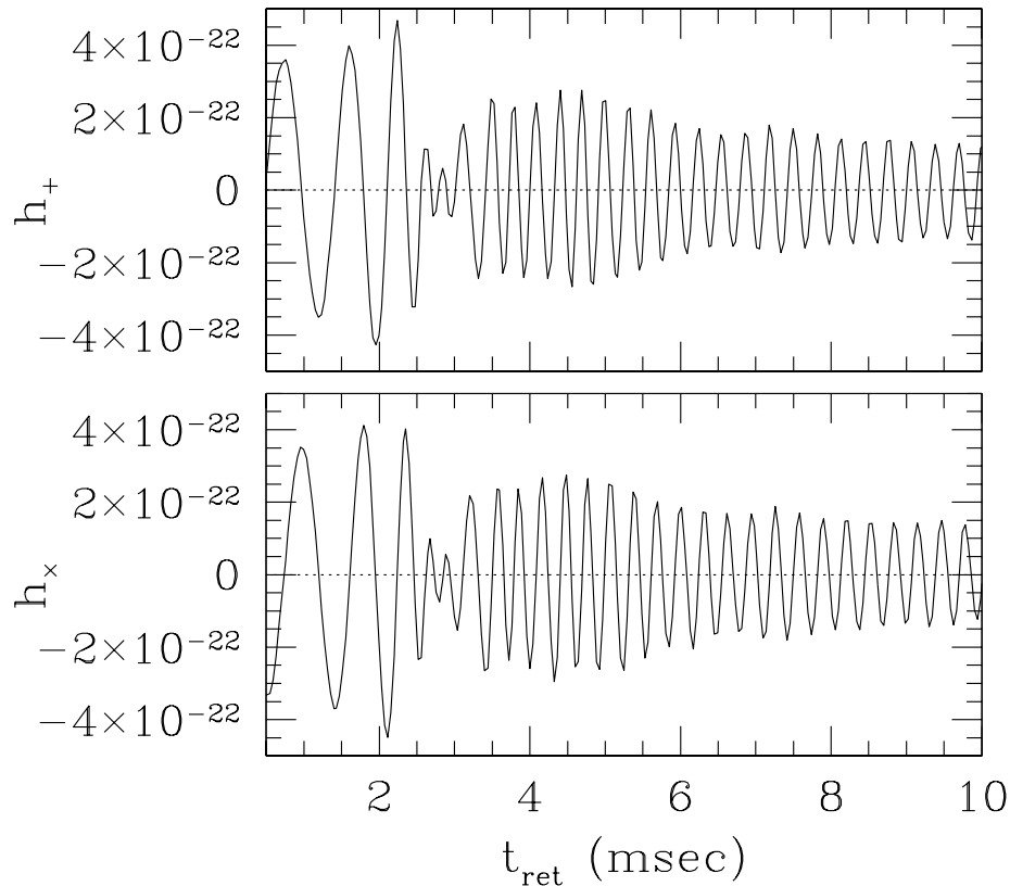
Figure 16.10: Waveforms for the binary merger that produced the ellipsoidal hypermassive neutron star remnant depicted in Figure 16.9. The observer is located along the rotational axis of the binary at a distance of 50 Mpc and t_{\text{ret}} is retarded time. [From Shibata (2005).]
