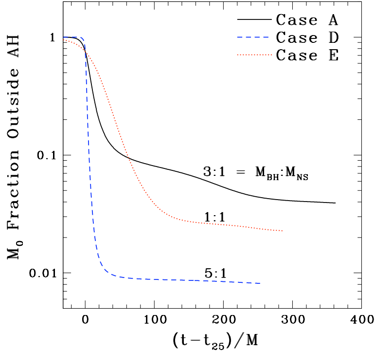
Figure 17.10: Rest-mass fraction outside the black hole as a function of time for irrotational binaries with different mass ratios. Here, the time coordinate is shifted by t_{25} , the time at which 25% of the neutron star rest mass has fallen into the apparent horizon. [From Etienne et al. (2009).]
