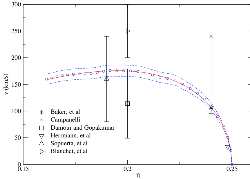
Figure 13.11: The kick velocity as a function of the symmetric mass-ratio parameter \eta = q/(1+q)^2 , where q is the ratio of irreducible masses. The line connecting the open circles, together with the dashed line marking a 6 % error, denote the results of González et al. (2007). Also plotted are the earlier numerical results of Baker et al. (2006); Campanelli (2005); Herrmann et al. (2007), as well as the analytical results of Blanchet et al. (2005); Damour and Gopakumar (2006); Soperueta et al. (2007). [From González et al. (2007).]
