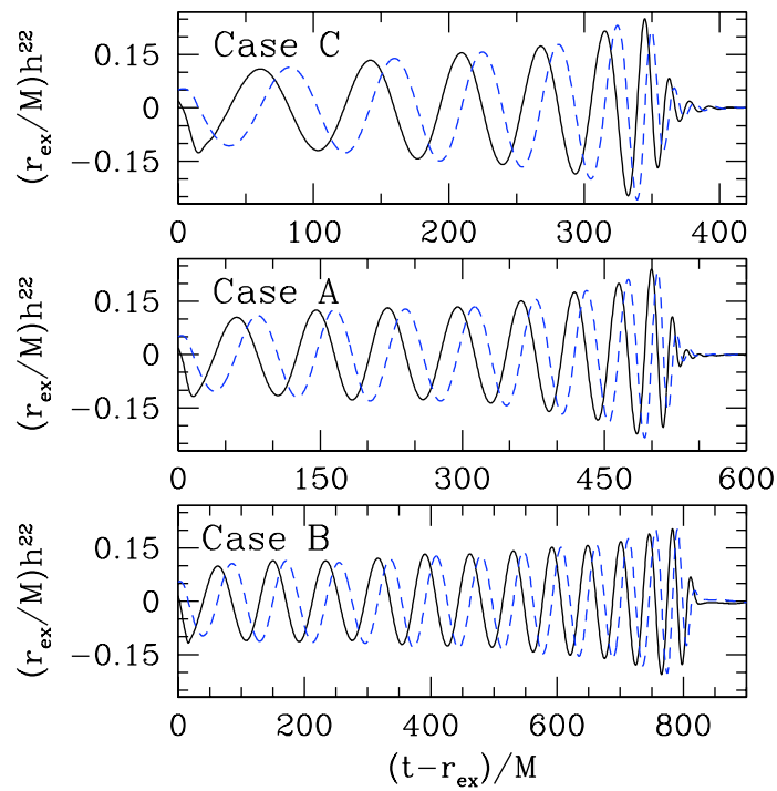
Figure 17.17: Gravitational wave signal for three binaries with mass ratio q = 3 initial black hole spins (top to bottom) J_{\text{BH}}/M_{\text{BH}}^2 = -0.5, 0 and 0.75 . The black solid (blue dash) line denotes the (2,2) mode of h_+ ( h_\times ) extracted at r_{\text{ex}} = 43.4M . [From Etienne et al. (2009).]
