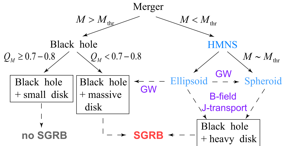
Figure 16.12: Plausible routes for the formation of a short-hard gamma-ray burst (SGRB) central engine following the merger of a binary neutron star. Here “HMNS” stands for hypermassive neutron star remnant and Q_M represents the mass ratio of the initial stars. For HMNS remnants, “GW versus B-field J-transport” denotes the outward transport of angular momentum dominated by gravitational wave emission versus magnetic torques. [From Shibata and Taniguchi (2006).]
