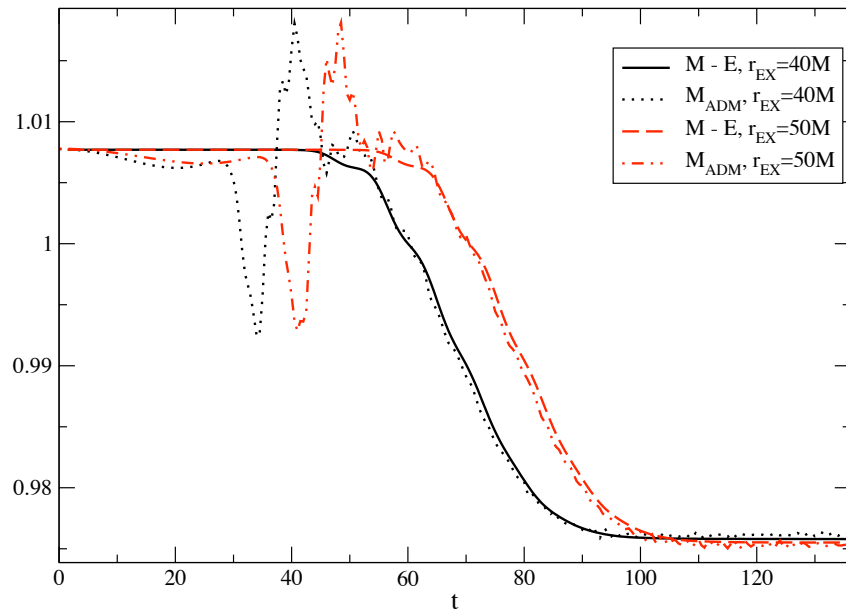
Figure 13.6: Demonstration of energy conservation in the calculation of Baker et al. (2006). The initial total energy (the initial total ADM mass) M minus the energy E carried off in gravitational radiation agrees with the instantaneous total energy M_{\text{ADM}} to high accuracy. [From Baker et al. (2006)].
