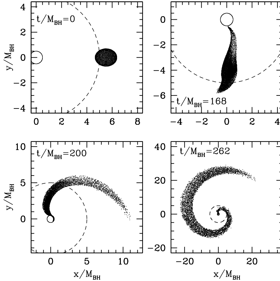
Figure 17.4: Snapshots of the disruption of a neutron star at selected times, projected into the orbital plane of the black hole-neutron star binary, as computed assuming conformally flat gravitation. The neutron star is an n = 1 polytrope with a compaction at infinite separation of M_{\text{NS}}/R_{\text{NS}} = 0.09 ; the binary mass ratio is M_{\text{BH}}/M_{\text{NS}} = 10 . The neutron star, represented by approximately 60,000 SPH particles, disrupts near the ISCO (dashed curve) to produce a mass-transfer stream that eventually wraps around the black hole horizon (solid curve) to form a torus. The initial orbital period is P/M_{\text{BH}} = 105 . [After Faber et al. (2006).]
