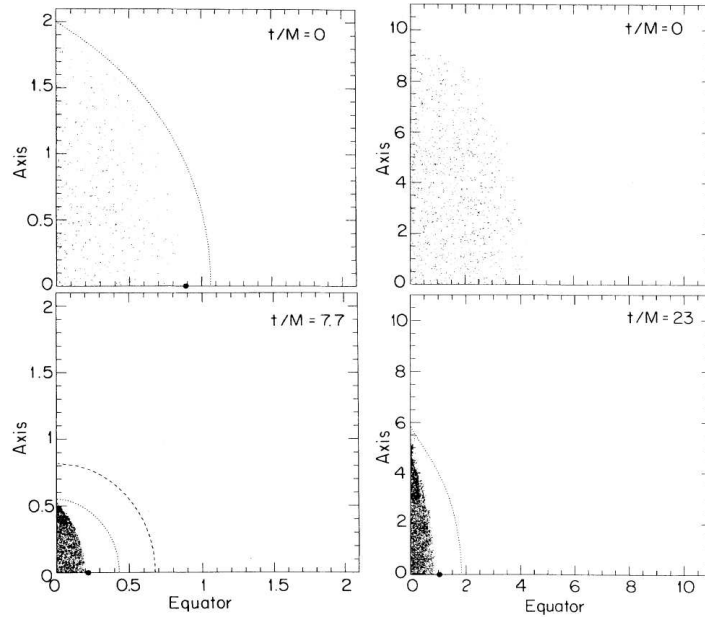
Figure 10.1: Left panels. Snapshots of the particle positions at initial and late times for prolate collapse. The positions (in units of M ) are projected onto a meridional plane. Initially the semi-major axis of the spheroid is 2M and the eccentricity is 0.9. The collapse proceeds non-homologously and terminates with the formation of a spindle singularity on the axis. However, an apparent horizon (marked by the dashed line) forms to cover the singularity. At t/M = 7.7 its area is \mathcal{A}/16\pi M^2 = 0.98 , close to the expected value of unity (gravitational radiation losses are negligible). Its polar and equatorial circumferences at that time are \mathcal{C}_{\text{pole}}^{\text{AH}}/4\pi M = 1.03 and \mathcal{C}_{\text{eq}}^{\text{AH}}/4\pi M = 0.91 . At later times these circumferences become equal and approach the expected value of unity. The minimum exterior polar circumference is shown by a dotted line and does not coincide with the matter surface. Likewise, the minimum equatorial circumference, which is a circle, is indicated by a solid dot. Here \mathcal{C}_{\text{eq}}^{\text{min}}/4\pi M = 0.59 and \mathcal{C}_{\text{pole}}^{\text{min}}/4\pi M = 0.99 . The formation of a black hole here is thus consistent with the hoop conjecture. Right panels. Snapshots of the particle positions at the initial and final times for prolate collapse with the same initial eccentricity as in the left panel but with initial semi-major axis equal to 10M . The collapse proceeds as in the left panel and terminates with the formation of a spindle singularity on the axis at t/M = 23 . The minimum polar circumference is \mathcal{C}_{\text{pole}}^{\text{min}}/4\pi M = 2.8 . There is no apparent horizon, in agreement with the hoop conjecture. This may be a candidate for a naked singularity. [From Shapiro and Teukolsky (1991b).]
