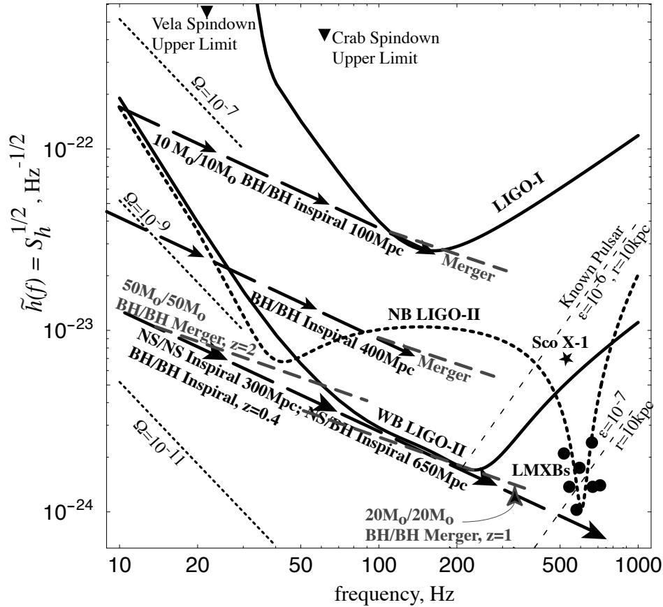
Figure 9.4: The noise curve \tilde{h}(f) for several planned LIGO Interferometers. Also included is the signal strength \tilde{h}_s(f) for a number of promising sources in the high-frequency band (see Section 9.2.1). Whenever a point on the signal curve lies above the interferometer's noise curve, the signal is detectable with a false alarm probability of less than one percent. [From Cutler and Thorne (2002).]
