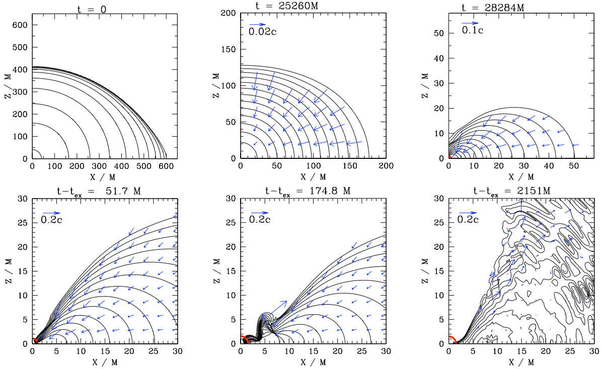
Figure 14.8: Snapshots of meridional rest-mass density contours and velocity vectors at selected times for n = 3 collapse. The initial model is rotating uniformly near the mass-shedding limit at the onset of gravitational instability to collapse. The density contour curves are drawn as follows: (a) Pre-excision top row, at t = 0 , \rho_0 = 10^{-i-0.1}\rho_{0c}(0) with j = 0, 1, \dots, 10 , where \rho_{0c}(0) is the initial central density; at t = 25260M , \rho_0 = \rho_{\text{scal}}10^{-0.3j} ( j = 0-12 ), where \rho_{\text{scal}} = 11\rho_{0c}(0) and at t = 28284M , \rho_{\text{scal}} = 1000\rho_{0c}(0) . (b) Post-excision bottom row, \rho_0 = 100\rho_{0c}(0)10^{-0.3j} ( j = 0-10 ). The thick solid (red) curve denotes the apparent horizon. For post-excision evolution, time is measured from the beginning of excision ( t_{\text{ex}} = 28284M ). Note that the coordinate scale decreases as time increases to show the central region in detail. [After Liu et al. (2007).]
