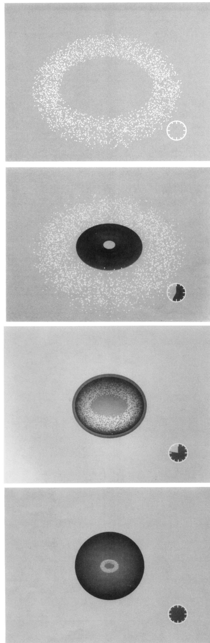
Figure 10.9: Three-dimensional views of the collapse of the rotating toroid shown in Figure 10.8. The images are viewed from 45^\circ above the equatorial plane. The first image shows the initial configuration. The remaining three images are at the same times as the last three images in Figure 10.8. The outermost shaded region is the event horizon, the shaded region inside it is the apparent horizon. The scale of the last three images is larger by a factor of 2 over the first image. The clock on the lower right denotes the fraction of time that has elapsed since the onset of the simulation. [From Hughes et al. (1994).]
