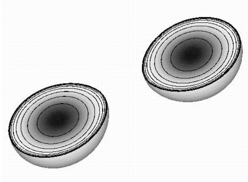
Figure 15.1: Rest-mass density contours in the equatorial plane for a neutron star binary orbiting close to the ISCO. These stars satisfy a polytropic equation of state with n = 1 , and each star has a rest mass of \bar{M}_0 = 0.169 , corresponding to a compaction in isolation of (M/R)_\infty = 0.175 . (The maximum-mass configuration in isolation has \bar{M}_0 = 0.180 and (M/R)_\infty = 0.215 .) The lines correspond to contours of constant rest-mass density in decreasing factors of 0.556. [From Baumgarte et al. (1998a).]
