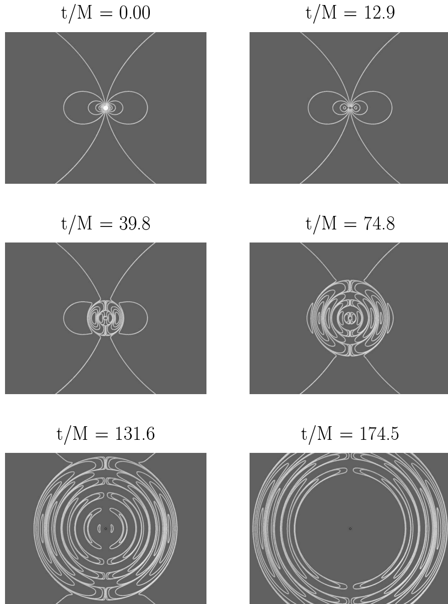
Figure 5.6: Far-zone view of the same collapse depicted in Figure 5.5. Note the transformation of the dipole field from a quasi-static longitudinal field to a transverse electromagnetic wave. [From Baumgarte and Shapiro (2003a).]
