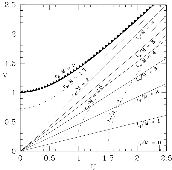
Figure 8.1: Slices of constant Schwarzschild time t_s for a spherical black hole, plotted in a Kruskal-Szekeres diagram. The dashed line denotes the event horizon at r_s/M = 2 and the sawtooth curve denotes the central singularity at r_s/M = 0 .
