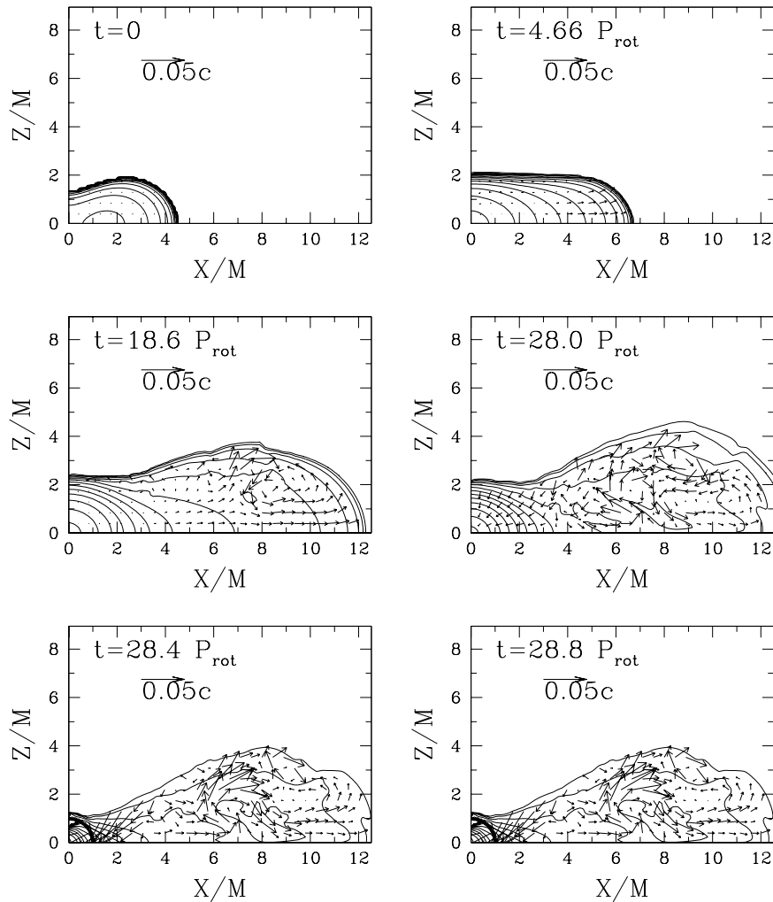
Figure 14.11: Meridional rest-mass density contours and velocity field at various times for a hypermassive star driven to catastrophic collapse by secular (viscous) redistribution of angular momentum. The simulation was performed by assuming that the system is axisymmetric and experiences no cooling. The levels of the contours (from inward to outward) are \rho_0/\rho_{0,\text{max}} = 10^{-0.15(2j+0.6)} , where j = 0, 1, \dots, 12 . In the lower right panel ( t = 28.8P_{\text{rot}} ), the thick curve denotes the apparent horizon. [From Duez et al. (2004).]
