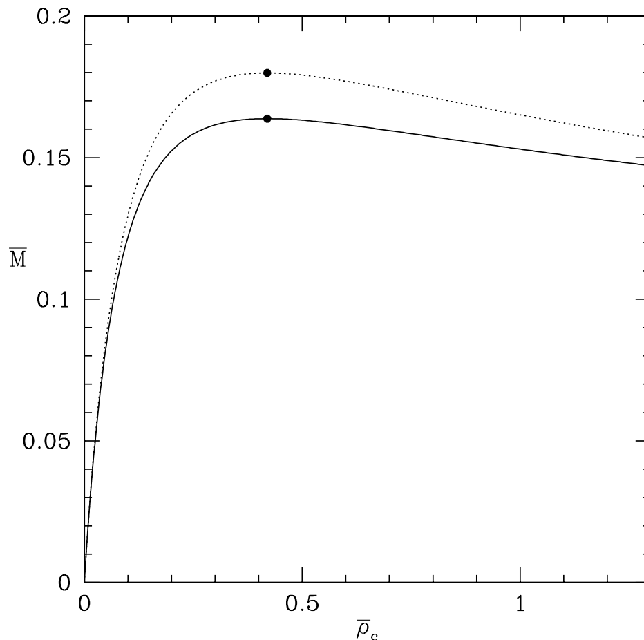
Figure 1.2: Equilibrium sequence for n = 1 spherical polytropes. The total mass-energy \bar{M} (solid line) and the rest-mass \bar{M}_0 (dotted line) are plotted as functions of the central mass-energy density \bar{\rho}_c along the sequence. The dots indicate the turning points, or the location of the maximum mass configuration, on each curve. The turning points occur at the same density along the two curves.
