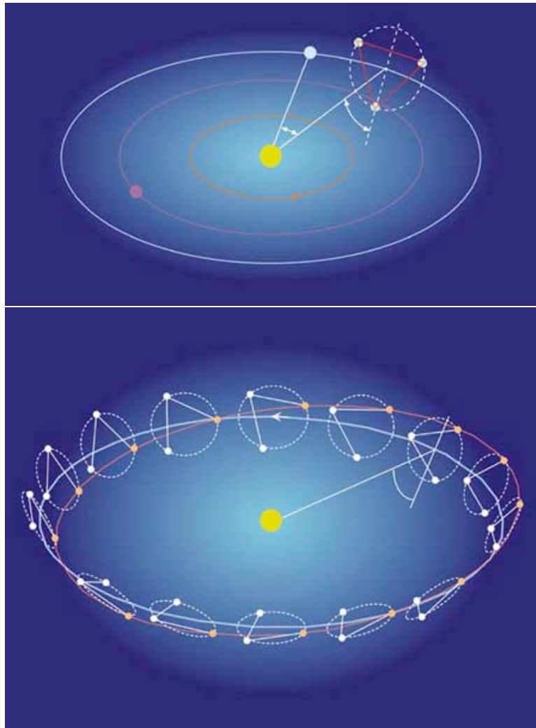
Figure 9.5: LISA’s orbit about the Sun. The top image shows how the triangle of three LISA spacecrafts trails Earth’s orbit about the Sun by 20^\circ . The bottom image follows one of the three satellites’ orbit about the Sun, demonstrating how the triangle’s orientation changes during the course of a year. [From LISA web site, http://lisa.nasa.gov .]
