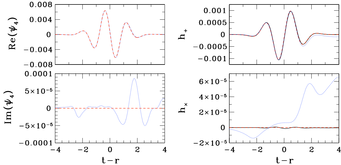
Figure 9.8: The left panels show the Weyl scalar \psi_4 for an even-parity l = 2 , m = 0 linearized wave at a point (r, \theta, \phi) = (6.0, 0.79, 0.52) . The dotted (blue) line shows numerical results, and the dashed (red) line analytical values. The right panels show the gravitational waveforms h_+ and h_\times for the same wave. The dashed (red) lines show the analytical waveforms (which are computed in Exercise 9.8), the solid (black) lines are the numerical waveforms based on the Moncrief formalism (computed from R_{20} , shown in Figure 9.7, using equation (9.109)), and the dotted (blue) line shows the numerical waveforms constructed from the Weyl scalar \psi_4 in equation (9.126).
