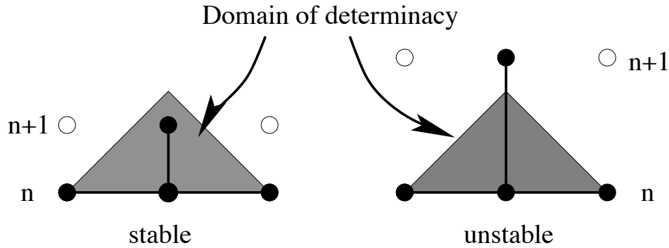
Figure 6.6: The Courant condition for many explicit finite difference implementations of hyperbolic equations requires the new grid point u_j^{n+1} to lie inside the domain of determinacy of the finite difference stencil on the previous time level n .
