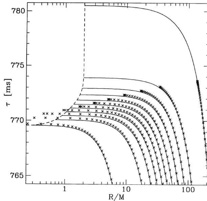
Figure 8.22: Comparison of simulations of the collapse of a slightly pressure-depleted 1.4M_{\odot} core with \rho_0 = 10^{12} and \gamma = 4/3 . Plotted is a spacetime diagram of the late-time evolution showing the world lines of Lagrangian mass shells obtained with a Hernandez-Misner code (solid lines) and a Misner-Sharp code (crosses). The dashed line marks the event horizon. [From Baumgarte et al. (1995)].
