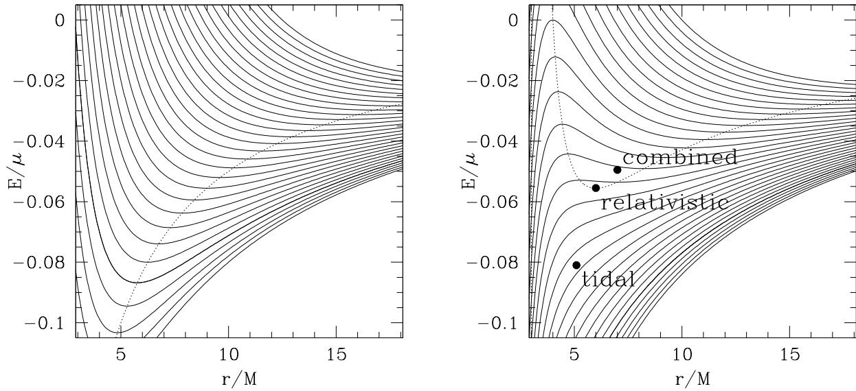
Figure 12.2: The energy E as a function of separation for a point-mass Newtonian binary (left panel), and a toy model problem that incorporates relativistic effects (right panel). The solid lines are contours of constant angular momentum J , with the values of J increasing from the bottom to the top. Extrema of these contours correspond to circular orbits (equation 12.9). The dashed line connects the circular orbits and represents the equilibrium energy E_{\text{eq}} . A turning point in this equilibrium energy represents the ISCO (equation 12.13) and is marked by dots for relativistic, tidal and combined relativistic and tidal effects. [From Baumgarte (2001).]
