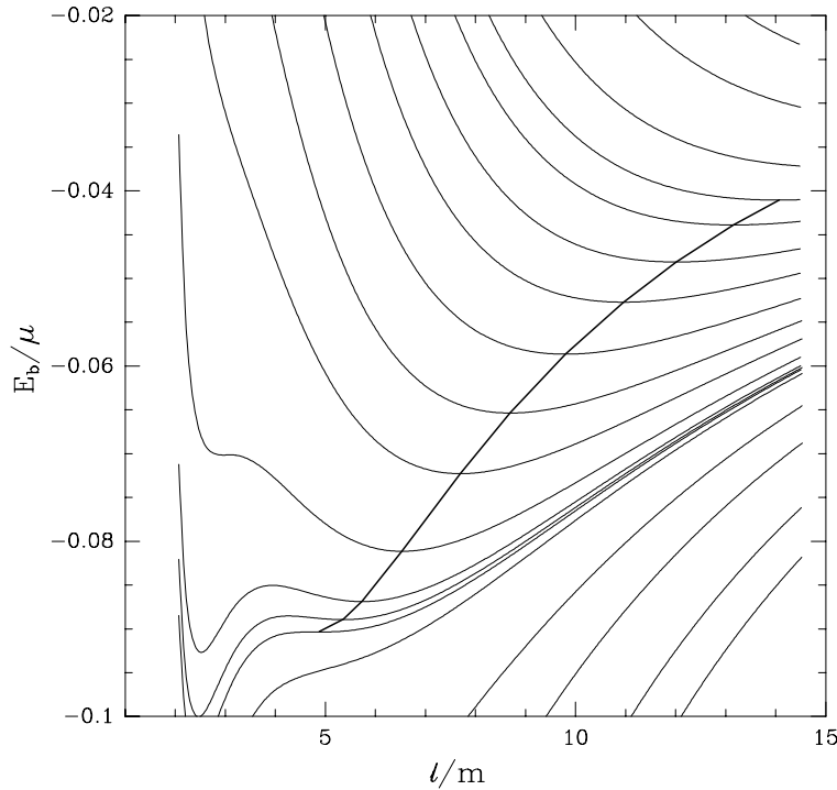
Figure 12.3: [CAMBRIDGE: replace m with M in label.] The binding energy E_b/\mu as a function of separation l for various values of the angular momentum J/\mu M (thin lines) as obtained by the Bowen-York conformal-imaging method for an equal mass, nonspinning black hole binary. The thick line connects a sequence of stable quasicircular orbits, which correspond to minima of the binding energy (equation 12.61), and yields E_{\text{eq}} as a function of l (“effective potential approach”). This sequence terminates at the ISCO, identified where a E_b curve at constant J exhibits a point of inflection. [From Cook (1994).]
