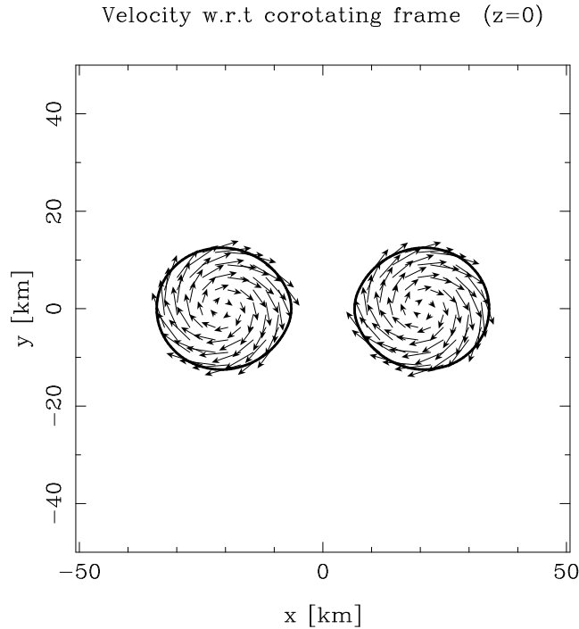
Figure 15.5: [CAMBRIDGE: remove header above figure] The internal velocity field with respect to the corotating frame in the orbital plane for identical stars of rest-mass M_0 = 1.625M_\odot at a coordinate separation of 41 km. The binary stars are irrotational and constructed from an n = 1 polytropic EOS with K = 1.8 \times 10^{-2} \text{Jm}^3\text{kg}^{-2} . The thick lines mark the stellar surfaces. [From Gourgoulhon et al. (2001).]
