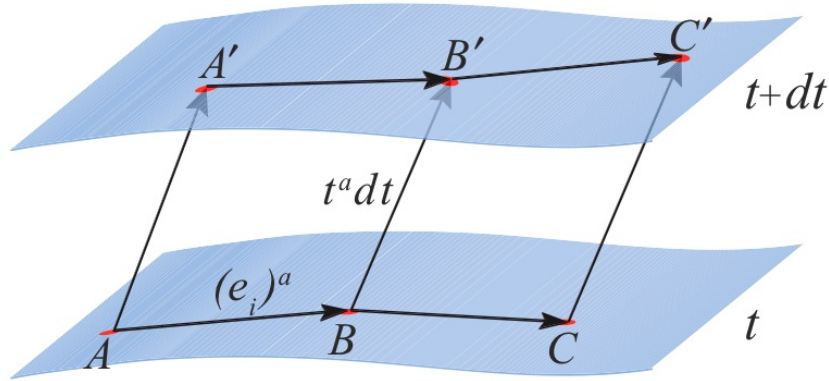
Figure 2.3: Spatial basis vectors e_{(i)}^a are Lie dragged from one spacelike slice to the next along the coordinate congruence t^a . Consequently, these basis vectors connect points with the same spatial coordinates on neighboring slices (e.g., points A , B and C on slice t have the same spatial coordinates as points A' , B' and C' , respectively, on slice t + dt ).
