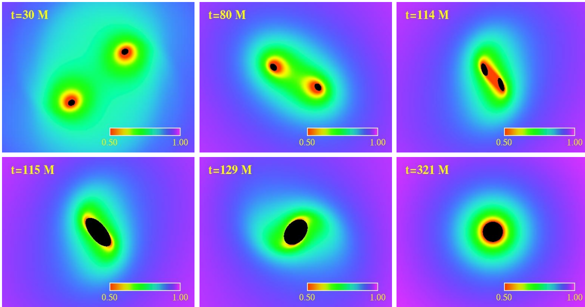
Figure 13.3: Evolution of the lapse function \alpha in the orbital plane during the merger of an equal-mass, nonspinning binary black hole in the calculation of Pretorius (2005a). The black regions are the excised domains in the black hole interior. The apparent horizons merge between the times of 114M and 115M , where M is the total initial ADM mass of the binary, and the initially distorted remnant subsequently settles down to an axisymmetric stationary Kerr black hole. [Figures provided by Pretorius, private communication.]
