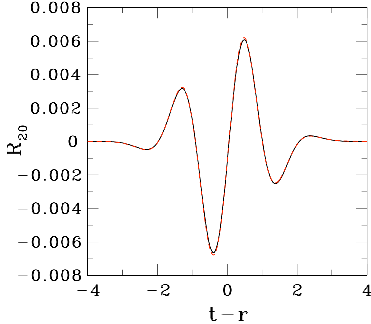
Figure 9.7: The Moncrief function R_{20} at r = 6.0 for a l = 2 , m = 0 linear wave. The solid (black) line denotes numerical results, and the dashed (red) line is the analytical value given by equation (9.93).
