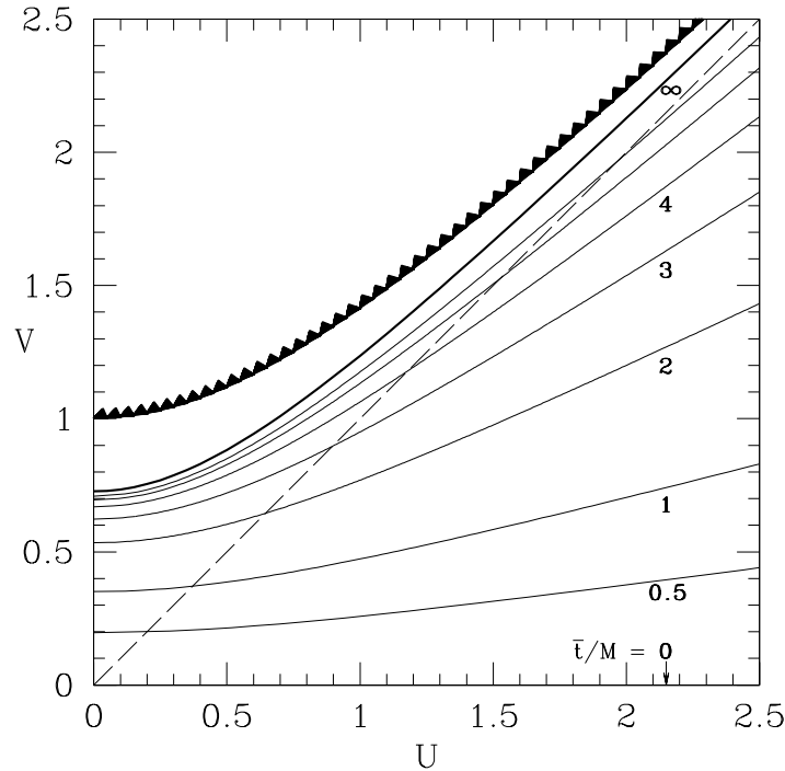
Figure 8.3: Maximal time slices of a Schwarzschild black hole, plotted on a Kruskal-Szekeres diagram. The dashed line denotes the event horizon at r_s/M = 2 , the sawtooth curve denotes the central singularity at r_s/M = 0 and the darker solid line shows the limiting slice at r_s = 3M/2 .
