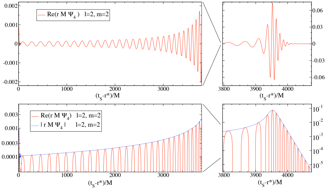
Figure 13.9: The gravitational waveform, extrapolated to spatial infinity, for an equal-mass, non-spinning, black hole binary. The top panel shows the real part of the dominant \ell = 2 , m = 2 mode of \psi_4 on the linear scale, the bottom panel on a logarithmic scale. The panels on the right show an enlargement of the data for the merger and ringdown. [From Scheel et al. (2009).]
