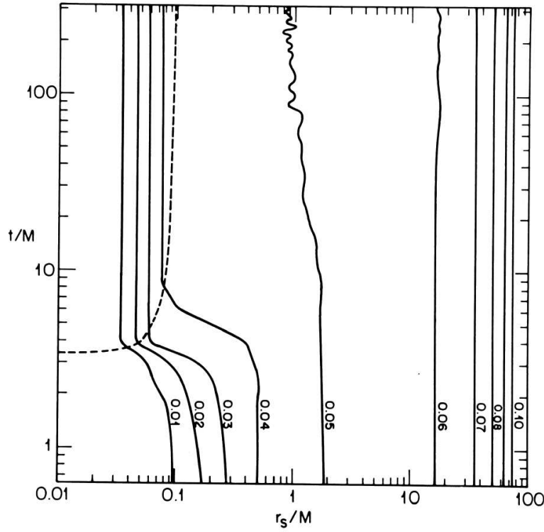
Figure 8.17: Spacetime diagram in polar slicing for the relativistic polytrope shown in Figure (8.16). Labelling is the same as in Figure (8.13). The event horizon asymptotes to r_s/M = 0.1 , at which point it encompasses 5% of the total cluster rest mass. [From Shapiro and Teukolsky (1986)].
