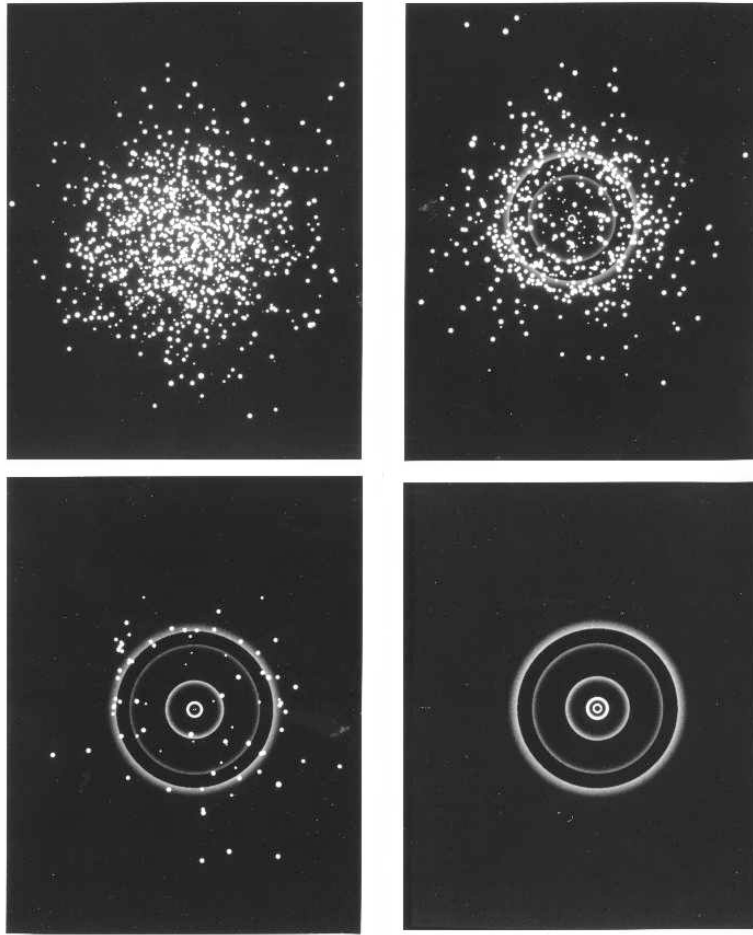
Figure 8.12: The collapse of a marginally unstable gas of collisionless particles of arbitrary mass M which at t = 0 obeys a truncated, isothermal Maxwell-Boltzmann distribution function with an areal radius R/M = 9 . Spherical flashes of light are used to probe the spacetime geometry; at late times the light rays are trapped by the gravitational field. Their trajectories help locate the black hole event horizon, which in this example eventually reaches r_s/M = 2 and encompasses all the matter. [From Shapiro and Teukolsky (1988)].
