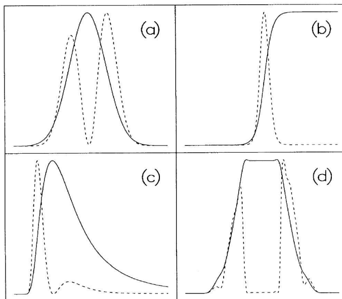
Figure 8.23: Typical initial profiles of the scalar field \varphi (solid lines) and the radial mass-energy density dm/dr (dotted lines) for four families of initial data considered by Choptuik. [From Choptuik (1993)].
