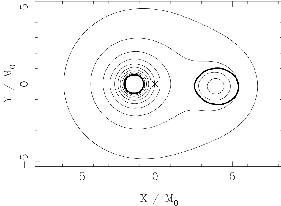
Figure 17.1: Contours of the conformal factor \psi in the equatorial plane for an irrotational binary black hole-neutron star close to tidal break-up. This binary has a mass ratio of q = 3 , and the neutron star, governed by a polytropic equation of state with polytropic index n = 1 , has a compaction of M_{\text{NS}}/R_0 = 0.1452 , where M_{\text{NS}} is the ADM mass that the star would have in isolation, and R_0 its areal radius. The circle on the left marks the black hole’s apparent horizon. The interior of this coordinate circle is excised from the computational grid. The other thick line on the right marks the neutron star’s deformed surface. The cross “ \times ” indicates the position of the rotation axis. [From Taniguchi et al. (2008).]
