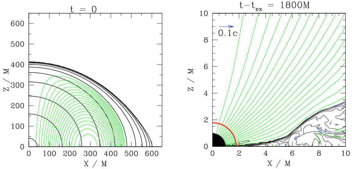
Figure 14.16: Snapshots of meridional rest-mass density contours (black), velocity vectors and magnetic field lines (green) for the initial and endpoint configurations for n = 3 magnetorotational collapse. The initial model is identical to the configuration in Figure 14.8 except that it is threaded by a poloidal magnetic field. Field lines coincide with contours of vector potential A_\varphi and are drawn for A_\varphi = A_{\varphi,\max}(j/20) with j = 1, 2, \dots, 19 where A_{\varphi,\max} is the maximum value of A_\varphi . In the final, post-excision model ( t_{\text{ex}} = 29150M ), the density levels are drawn for \rho_0 = 100\rho_{0c}(0)10^{-0.3j} ( j = 0-10 ). The thick (red) line near the lower left corner denotes the apparent horizon. [After Liu et al. (2007).]
