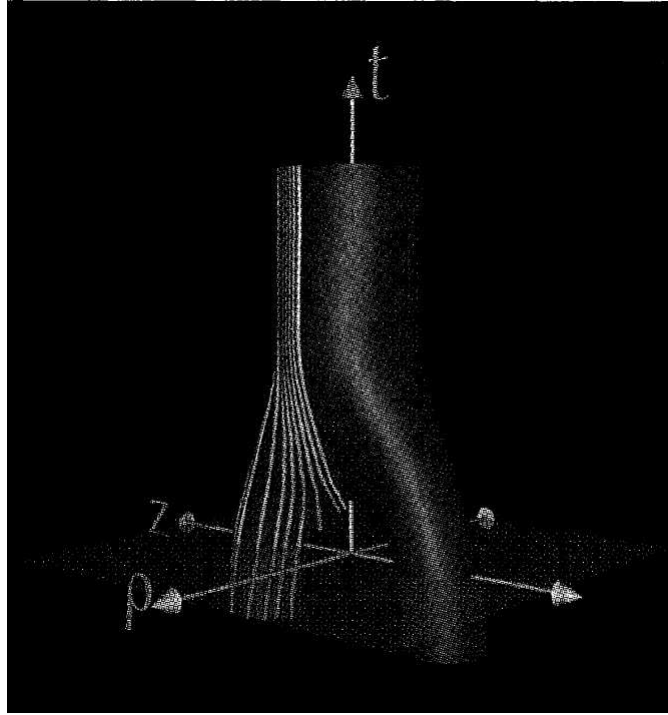
Figure 7.2: The “pair of pants” formed by the event horizon in a spacetime diagram depicting the head-on collision of two “eternal” black holes [From Matzner et al. (1995)].
