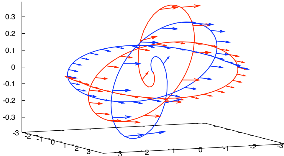
Figure 13.14: Puncture trajectories together with black hole spin directions, shown at time intervals of 4M . The initial orbital plane is in the x - y (horizontal) plane, and the initial black hole spins reside in this plane, both pointing in the positive y -direction (to the right). During the course of the inspiral the spins rotate by approximately 90^\circ within the orbital plane, and also pick up a nonzero z component orthogonal to the orbital plane. Simultaneously the orbital plane tilts, leaving a remnant with an angular momentum that has nonzero components in both the y and z directions. Note that the z -scale is 1/10 th the x and y -scale. [From Campanelli et al. (2007).]
