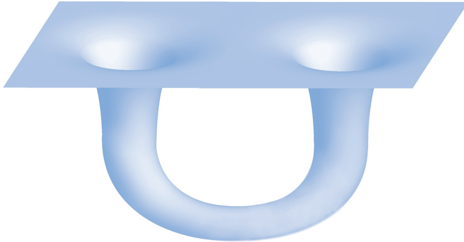
Figure 3.4: Illustration of a wormhole black hole solution.
