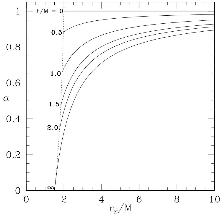
Figure 8.4: The lapse \alpha as a function of areal radius r_s on selected maximal slices.
