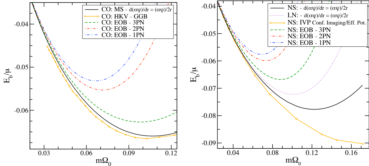
Figure 12.6: [CAMBRIDGE: replace \Omega_0 with \Omega_{\text{orb}} and m with M in label] The binding energy E_b versus the orbital angular velocity \Omega_{\text{orb}} for corotational (left panel) and nonspinning (right panel) equal-mass binaries. The solid lines mark the results of Cook and Pfeiffer (2004) and Caudill et al. (2006), computed in the conformal thin-sandwich formalism with the equilibrium black-hole boundary conditions of Section 12.3.2 for corotating and exactly nonspinning black holes. The dotted line labeled “LN” in the right panel was obtained similarly, except that the black holes are nonspinning to leading order only. The solid dotted line labeled “CO: HKV-GGB” in the left panel marks the results of Grandclément et al. (2002), who use an approximate isometry boundary condition on the horizon. The solid dotted line labeled “NS: IVP” marks the results from the Bowen-York effective potential approach, using the conformal imaging technique (Cook, 1994). Finally, the dashed and dashed-dotted lines denote post-Newtonian “effective one-body” results (Damour et al., 2002). [From Cook and Pfeiffer (2004) and Caudill et al. (2006).]
