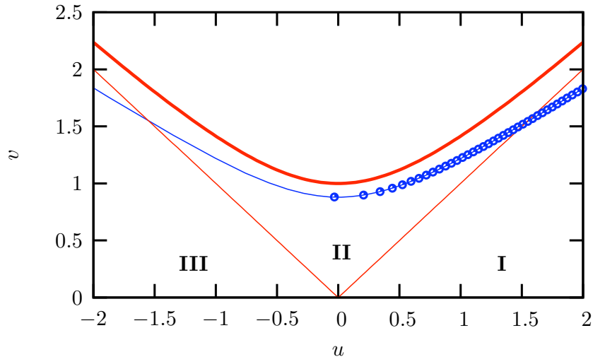
Figure 13.2: The spatial slice at t = 3M in a moving puncture simulation of a single Schwarzschild black hole, plotted in a Kruskal-Szekeres diagram. The solid blue line shows the slice that results from an evolution with zero shift in equation (13.3), while the dots represent the location of individual grid points when evolved with the \Gamma -driver condition (4.83). The thick upper red line represents the spacetime singularity at r_s = 0 . [After Brown (2008).] [CAMBRIDGE: change the upper red line to a sawtooth, as in Figs 1.1 or 8.1]. Change fig caption accordingly.]
