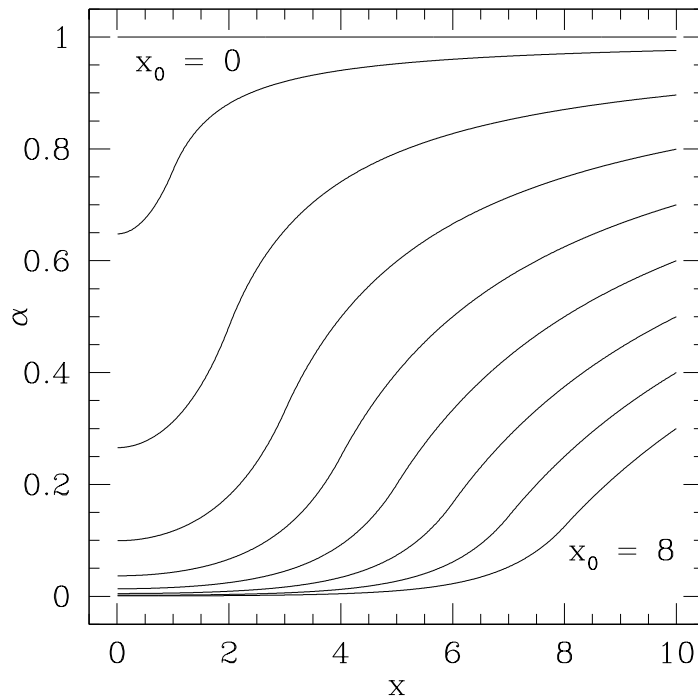
Figure 4.2: The lapse \alpha as a function of dimensionless radius x for select values of the parameter x_0 , plotted according to the analytic model. The parameter x_0 varies between x_0 = 0 (top curve, \alpha = 1 ) and x_0 = 8 (bottom curve) in increments of unity. The “collapse of the lapse” is evident in the strong-field region. (After Smarr and York (1978a).)
