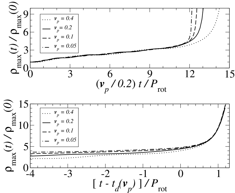
Figure 14.12: Scaling behavior exhibited by the evolution of the maximum rest-mass density of a hypermassive star for different strengths of viscosity, assuming rapid cooling. Upper panel: the curves coincide when plotted against the scaled time during secular evolution prior to dynamical collapse at t_d(\nu_p) . Lower panel: during dynamical collapse, it is possible to shift the time axes [t \rightarrow t - t_d(\nu_p)] so that the curves again coincide, which indicates that viscosity plays an insignificant role during the dynamical collapse phase. [From Duez et al. (2004).]
