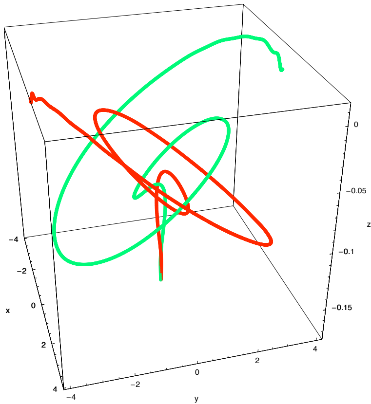
Figure 13.12: Coordinate trajectories of the black hole centers (punctures) for an equal-mass, spinning black hole binary. The initial spins are both perpendicular to the orbital angular momentum; each spin vector points away from the companion along the line joining the centers. Following merger, the remnant receives a kick in the negative z -axis, perpendicular to the orbital plane. [From González et al. (2007).]
