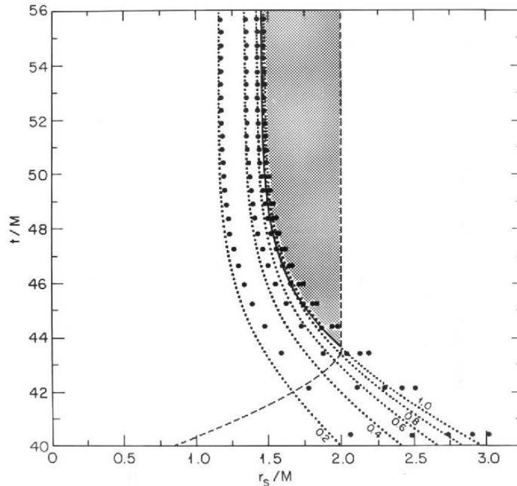
Figure 8.10: Spacetime diagram at late times for Oppenheimer-Snyder collapse in maximal slicing from R = 10M . The dotted lines are worldlines of Lagrangian matter elements from exact integrations. Each worldline is labelled by the fixed interior rest-mass fraction. The dots are points for the corresponding elements obtained with the numerical code. The dashed line is the event horizon. The shaded area is the region of trapped surfaces. Its outer boundary, the apparent horizon, coincides with the event horizon. Its inner boundary is just inside the surface of the matter. [From Shapiro and Teukolsky (1985b)].
