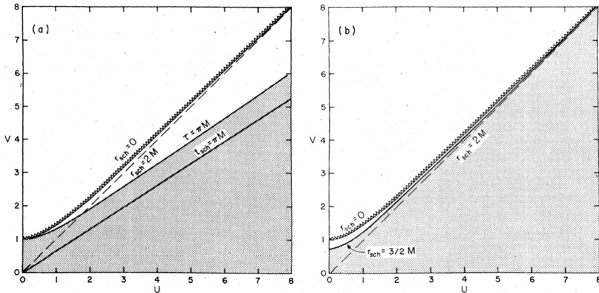
Figure 4.1: [CAMBRIDGE: Change label r_{\text{sch}} to r_s in Figures.] The shaded regions on the Kruskal-Szekeres diagrams represent the development of the initial v = 0 time slice in a Schwarzschild spacetime for geodesic slicing in the left panel (a) and maximal slicing in the right panel (b). The geodesic slices hit the singularity at (areal) radius r_s = 0 after a coordinate time t = \pi M (= proper time for any normal observer), during which only a small fraction of the black hole exterior is covered. The maximal slices, on the other hand, cover the entire black hole exterior and approach a limiting surface at r_s = (3/2)M in the interior as t \rightarrow \infty . (After Smarr and York (1978a).)
