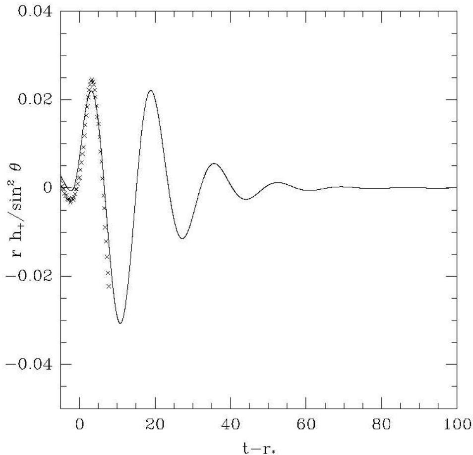
Figure 10.7: The gravitational waveform computed using the perturbation method for disk collapse is plotted as a function of retarded time in units of M . For comparison, the gravitational waveform computed at a radius r/M = 8 using a standard spacelike radiation extraction technique is also shown (crosses). [From Abrahams et al. (1995).]
