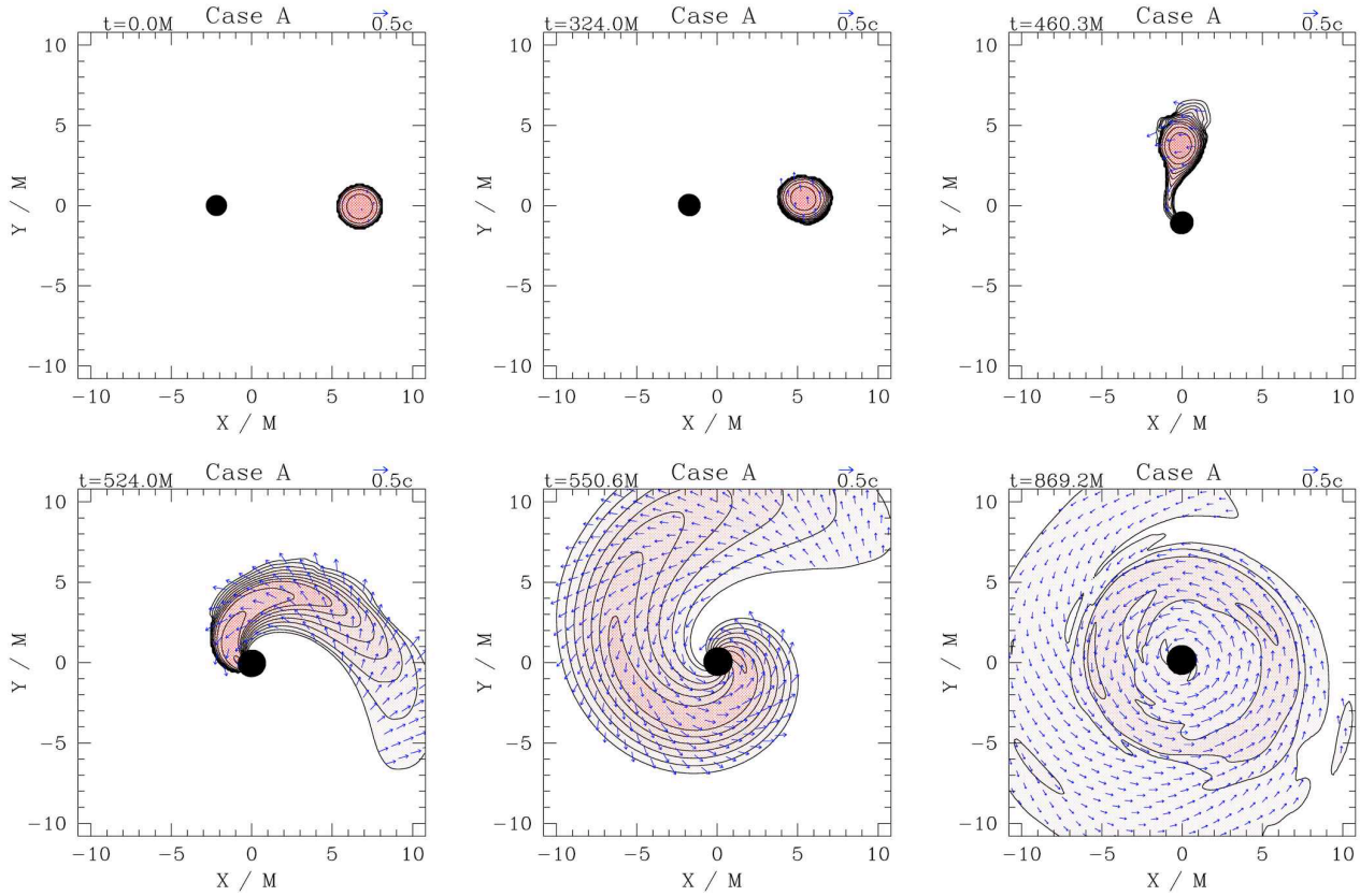
Figure 17.9: Snapshots of rest-density contours and 3-velocity vectors at selected times during the merger of the irrotational black hole-neutron star binary with mass ratio q = 3 shown in Figure 17.8 (case A). The contours represent the density in the orbital plane, plotted according to \rho_0 = \rho_{0,\max} 10^{-0.38j-0.04} , ( j=0, 1, \dots, 12 ), with darker grey scaling for higher density. The maximum initial neutron density is K\rho_{0,\max} = 0.126 , where K is the initial polytropic gas constant, or \rho_{0,\max} = 9 \times 10^{14} \text{g cm}^{-3} (1.4M_\odot/M_0)^2 . Arrows represent the velocity field in the orbital plane. The apparent horizon interior is marked by a filled black circle. In cgs units, the initial ADM mass for this case is M = 2.5 \times 10^{-5} (M_0/1.4M_\odot) s = 7.6 (M_0/1.4M_\odot) \text{km} . [From Etienne et al. (2009).]
