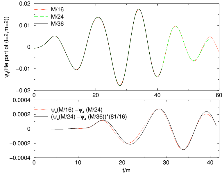
Figure 13.5: The gravitational waveform \text{Re}(\psi_4) for an equal-mass, nonspinning binary black hole merger in the calculation of Campanelli et al. (2006). Results are plotted for different grid resolutions. This convergence test suggests fourth-order convergence, as expected from a fourth-order finite-difference implementation [From Campanelli et al. (2006)].
