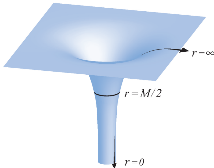
Figure 13.1: A schematic embedding diagram of a maximally sliced Schwarzschild geometry with C = 3\sqrt{3}M^2/4 (for t = \text{constant} and \theta = \pi/2 ; see equations 4.23 – 4.25). In contrast to the “wormhole” solution shown in Fig. 3.1, this “trumpet” solution has only one asymptotically flat end, while the other end, corresponding to r \rightarrow 0 , approaches an infinitely long cylinder of areal radius r_s = 3M/2 . [After Hannam et al. (2008).]
