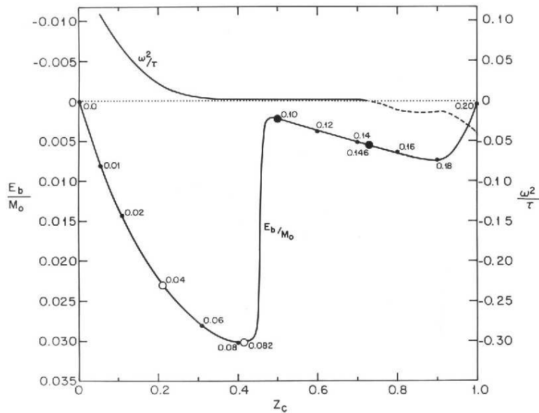
Figure 8.19: The fractional binding energy E_b/M and oscillation frequency \omega^2 in units of \tau = \rho_c - P are plotted as functions of central redshift Z_c for the n = 4 polytropic sequence. Clusters along the sequence are labelled by their value of the relativity parameter \alpha as defined in Fackerell (1970). The dynamical fates of four models along the sequence, as determined by numerical simulation, are as follows: open circles indicate stable equilibrium; filled circles indicate collapse to a black hole. [From Shapiro and Teukolsky (1985a)].
