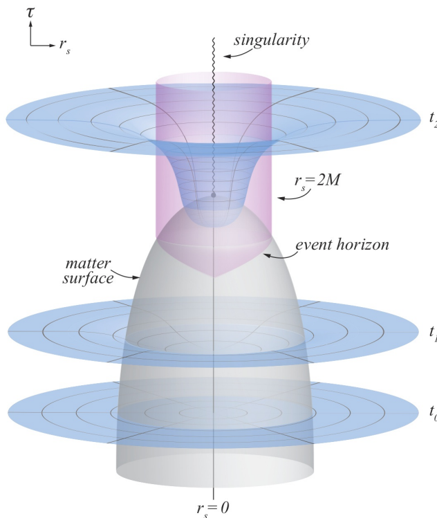
Figure 8.8: Schematic spacetime diagram of the collapse of a collisionless cluster to a black hole. The vertical axis measures proper time \tau measured by a normal observer and the horizontal axis measures areal (Schwarzschild) radius r_s . A singularity forms at the center in a finite proper time. The time slicing chosen here avoids the singularity by “slowing down” the advance of proper time near the center, hence the warping there of the spatial hypersurfaces with increasing coordinate time t . Spherical polar coordinate lines appearing on each slice mark the spatial grid, with the radial grid based on an isotropic coordinate r . When the spatial metric on the time slice t has the “radial” form A_s^2 dr_s^2 + r_s^2 d\Omega^2 , a spike develops in A_s near the event horizon, as in the usual static Schwarzschild geometry. When the isotropic metric A^2 dr^2 + A^2 r^2 d\Omega^2 is used, no spike appears. However, considerable radial grid must be expended along the throat near the horizon to determine the metric accurately (“grid stretching”). [After Shapiro and Teukolsky (1986)].
