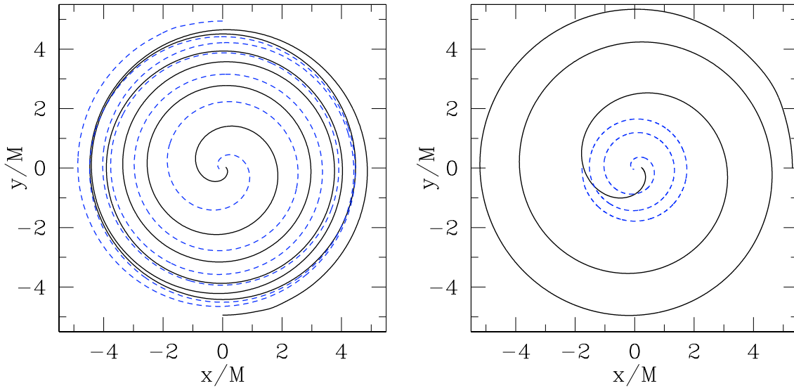
Figure I.1: Trajectory of the coordinate centroid of the “+” (black solid line) and “-” (blue dash line) black hole during nonspinning binary black hole inspiral and merger. The left-hand panel is the equal-mass case, the right-hand panel in the unequal mass case. [From Etienne et al. (2009).]
