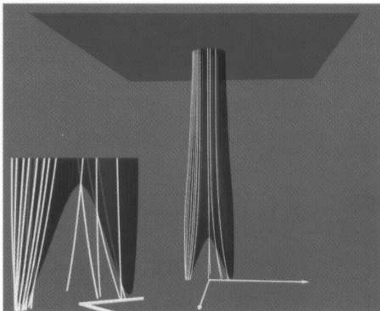
Figure 10.5: Spacetime diagram for the collision depicted in Figure 10.4. The diagram shows some of the null generators of the horizon. The time axis is vertical, the collision axis goes from left to right; one of the spatial dimensions is suppressed. The inset on the left zooms in on the caustic and crossover structure at the birth of the event horizon. [From Matzner et al. (1995).]
