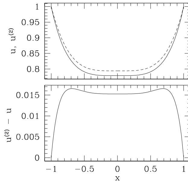
Figure 6.11: The top panel shows the exact solution u(x) (solid line) and the spectral solution u^{(2)}(x) (dashed line) to the differential equation (6.100), subject to boundary conditions (6.101). The bottom panel shows the absolute error u^{(2)}(x) - u(x) .
