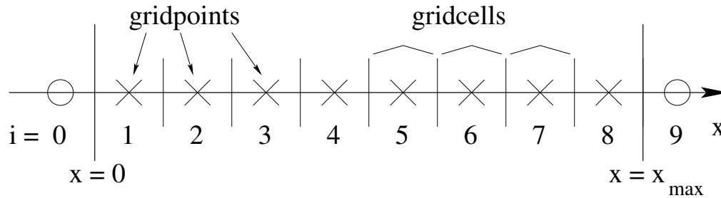
Figure 6.2: A cell-centered grid with 8 grid points. The virtual grid points 0 and 9 lie outside of the domain between x = 0 and x = x_{\max} and do not need to be allocated in the computational grid.
