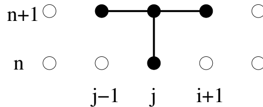
Figure 6.7: Finite difference stencil for the leap-frog scheme.
