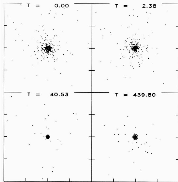
Figure 8.16: Snapshots of the central regions r_s/M \leq 2 during the collapse of the extreme core-halo configuration shown in Figure (8.15). The markers on frames are placed at intervals of \Delta r_s = 1M . The times are labelled by T \equiv t/M . The circle in the last frame shows the event horizon at r_s/M = 0.1 . The collapse of the innermost regions to a black hole is evident. By t/M \approx 40 , the cluster reaches a quasistationary state consisting of central black hole surrounded by a massive halo of orbiting particles. [From Shapiro and Teukolsky (1986)].
