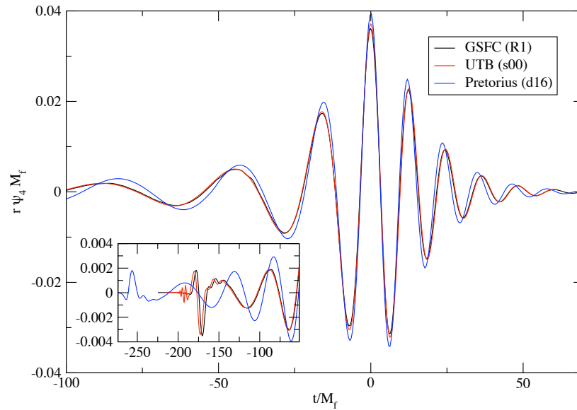
Figure 13.8: Comparison of the gravitational waveforms \text{Re}(\psi_4) obtained by three independent research groups: Pretorius (Pretorius (2005a); Buonanno et al. (2007)), Goddard Space Flight Center (GSFCC, e.g., Baker et al. (2006)) and University of Texas at Brownsville (UTB, e.g., Campanelli et al. (2006)). [From Baker et al. (2007).]
