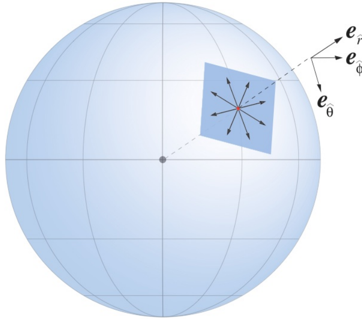
Figure 8.7: Schematic representation of the distribution of particles in a spherical cluster (see text). [After Shapiro and Teukolsky (1992b)].
