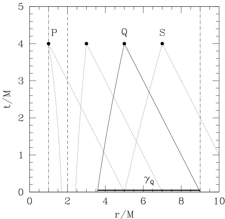
Figure 6.1: Backwards characteristics through several events in the Kerr-Schild metric of a Schwarzschild black hole. The interval \gamma_Q is the domain of dependence of the event Q ; the cone defined by \gamma_Q and Q is the domain of determinacy of the interval \gamma_Q . The dashed line tracks the event horizon, and the dashed-dotted lines mark some hypothetical computational boundaries.
