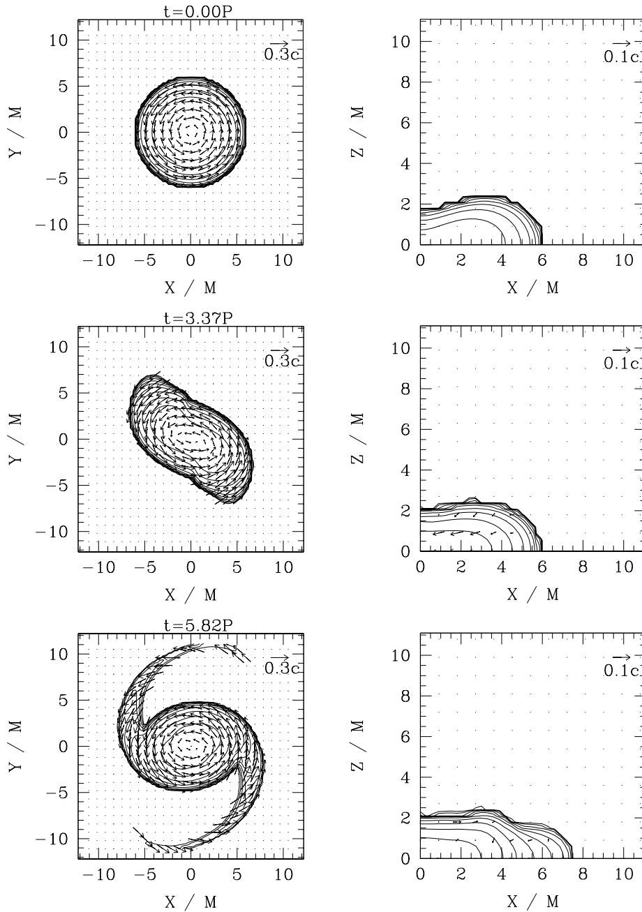
Figure 14.6: Snapshots of contours for the density \rho_* and the velocity field v^i in the equatorial plane (left) and in the meridional plane (right) for a bar-unstable model with R/M \approx 7.1 and \beta \approx 0.26 . The contour lines are drawn for \rho_*/\bar{\rho}_*_{\max} = 10^{-0.3j} for j = 0, 1, 2, \dots, 10 where \bar{\rho}_*_{\max} is 0.126, 0.172 and 0.264 at the three different times. The lengths of arrows are normalized to 0.3c (left) and 0.1c (right). The time is shown in units of the initial central period P \approx 15M . [From Shibata et al. (2000b).]
