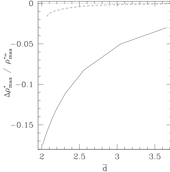
Figure 15.3: The relative change in the maximum density \Delta\rho_{\max}^*/\rho_{\max}^{*\infty} as a function of the separation \bar{d} between the locations of the maximum densities in an equal-mass, n = 1 polytropic binary with companions of rest-mass \bar{M}_0 = 0.18 (close to the maximum allowed mass for static stars). The solid line marks the changes in the density for corotational binaries, and the dashed line for irrotational binaries. The dotted lines marks \Delta\rho_{\max}^* = 0 . This graph shows that the central density decreases with decreasing binaries for both corotational and irrotational binaries. Similar results hold for binaries of different masses and polytropic indices, and also for unequal-mass binaries. [After Taniguchi and Gourgoulhon (2002).]
