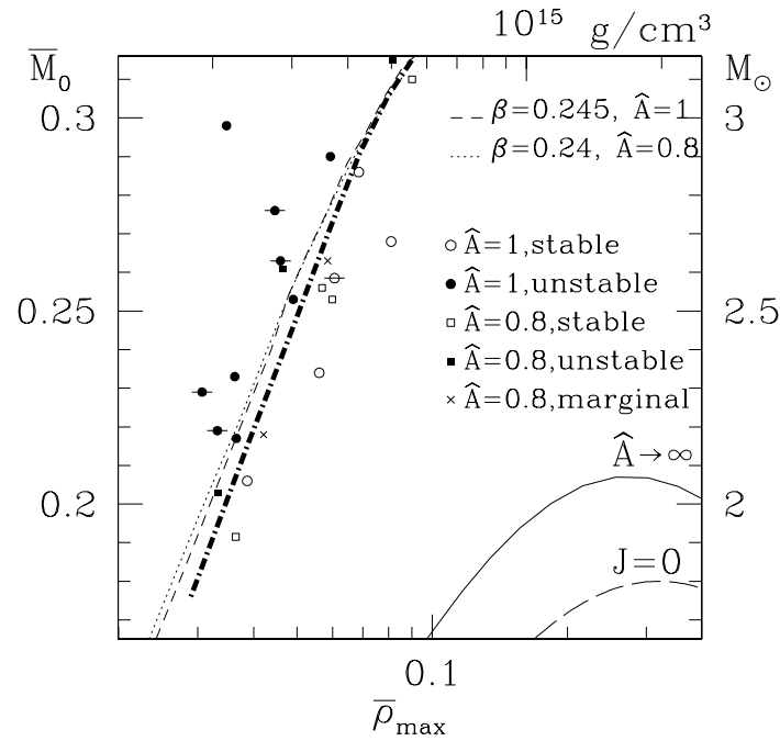
Figure 14.5: Models of differentially rotating stars in a \bar{M}_0 versus \bar{\rho}_{\max}^* diagram. Circles denote stars with \hat{A} \equiv A/R_e = 1 , squares with \hat{A} = 0.8 . Solid (open) circles or squares represent stars that are unstable (stable). Marginally stable stars are denoted with a cross. The region for the stable stars is clearly separated from that for the unstable stars by the thick dashed-dotted line. This line is followed fairly closely by the dashed and dotted lines, which have been constructed for differentially rotating stars of (\hat{A}, \beta) = (1, 0.245) and (0.8, 0.24) . The long-dashed and solid lines in the lower right-hand corner are for nonrotating spherical stars and rigidly rotating stars at the mass shedding limit. Scales for the top horizontal and right vertical axes are shown for polytropic constant K = 100(G^3 M_\odot^2/c^4) , for which the maximum rest mass for spherical stars is about 1.8M_\odot . [From Shibata et al. (2000b).]
