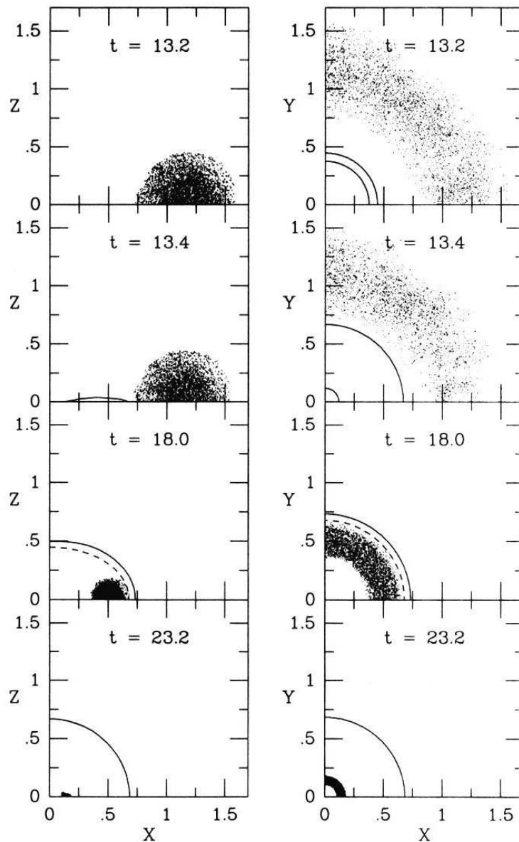
Figure 10.8: Snapshots of the collapse of a rotating toroid of collisionless particles at selected times. The left panels display meridional slices, the right panels show the equatorial plane. The solid line denotes the event horizon, the dashed line the apparent horizon. The earliest times shown occur soon after the appearance of the toroidal event horizon. By the final time shown here, the event and apparent horizons coincide. The coordinate labels (t, x, y, z) are in units of M . [From Hughes et al. (1994).]
