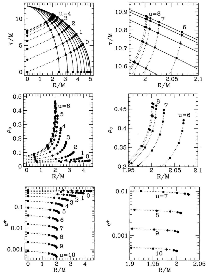
Figure 8.21: Oppenheimer-Snyder collapse of a star with initial compaction R/M = 5 . Shown are a spacetime diagram with world lines of selected mass shells (top row), rest-density profiles (middle row) and lapse function profiles (bottom row) at different observer times u . The analytic solution is represented by solid lines (world lines of mass shells) and dashed lines (lines of constant u ), while numerical results are represented by dots. [From Baumgarte et al. (1995).]
