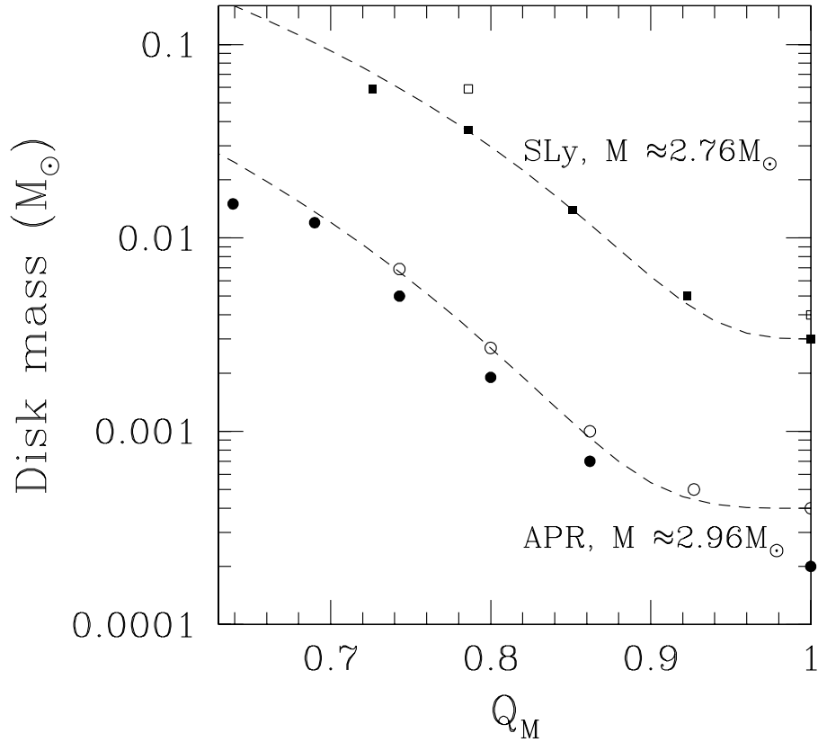
Figure 16.11: Baryon rest mass of the disk around the black hole as a function of the mass ratio Q_M in the case of prompt black hole formation. The disk mass is evaluated 0.5 ms after the appearance of an apparent horizon. The open circles and squares denote the results with 633 \times 633 \times 317 zones for the APR and SLy EOSs, respectively; the filled circles and squares denote the results with 377 \times 377 \times 189 zones. The results for the APR and SLy EOSs are obtained for a total initial binary ADM mass of M \approx 2.96M_\odot and 2.76M_\odot , respectively. [From Shibata and Taniguchi (2006).]
