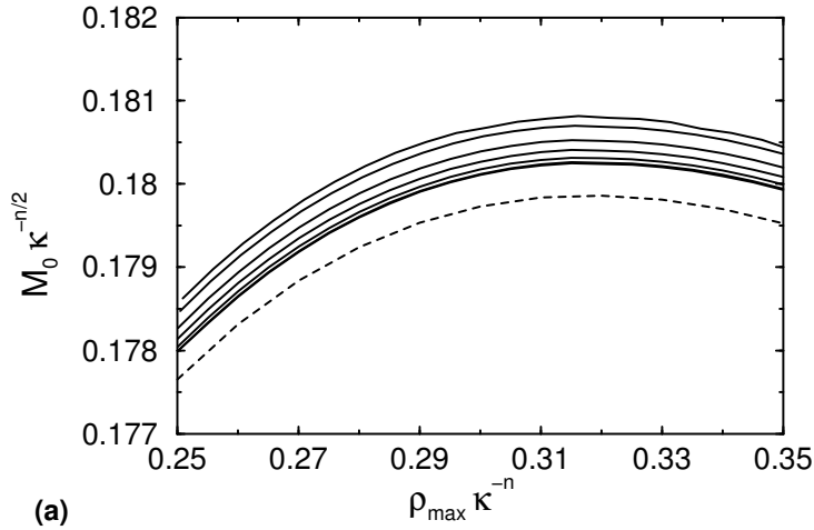
Figure 15.6: [CAMBRIDGE: change \rho_{\max} to \bar{\rho}_{0,\max} , M_0 to \bar{M}_0 , and remove \kappa altogether, as well as “(a)”.] The rest mass \bar{M}_0 as a function of maximum density \bar{\rho}_0 for separations \bar{d} = 1.3125, 1.375, 1.5, 1.625, 1.75, 1.875 and 2 (thick lines running from top to bottom) of irrotational, binary neutron stars constructed from an n = 1 polytropic EOS. The dashed line is the Oppenheimer-Volkoff result. [From Uryū et al. (2000).]
