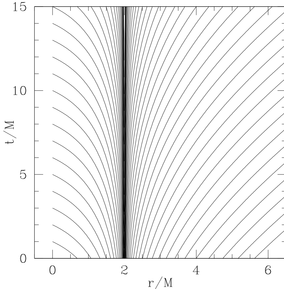
Figure 7.1: Worldlines of outgoing null geodesics in a Schwarzschild spacetime in Kerr-Schild coordinates (see Exercise 6.3). Traced backwards in time, these rays are strongly attracted to the event horizon at r/M = 2 . These worldlines coincide with contours of the function f introduced in equation (7.8).
