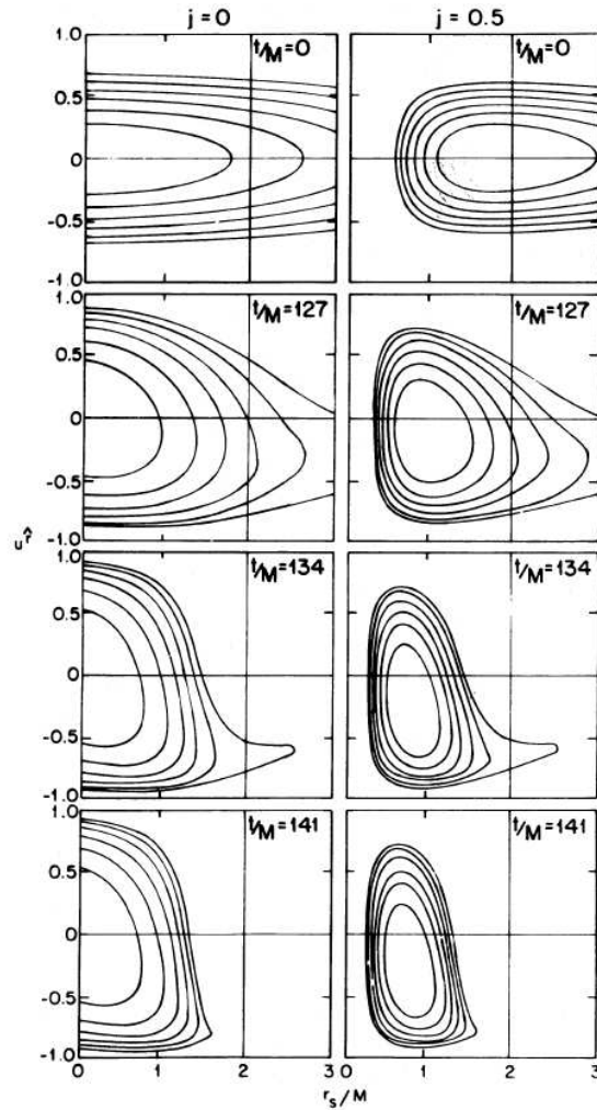
Figure 8.20: Time evolution of the distribution function f for the Maxwell-Boltzmann cluster. The areal radius r_s (in units of M ) and the radial velocity v^{\hat{r}} are used as phase space coordinates. Each plane (r_s, v^{\hat{r}}) is a two-dimensional slice taken from the three-dimensional phase space by setting the particle angular momentum j equal to a constant. The series on the left corresponds to j = 0 , while that on the right corresponds to j = 0.5M^2 , representing the angular momentum of a “typical particle” in this cluster ( 0 \leq j \lesssim M^2 for f \neq 0 ). Lines of constant f are shown, equally spaced between 0 and its maximum value on the slice. Note that for j \neq 0 , the matter never reaches r_s = 0 . In the final plots, the entire mass of the cluster has collapsed inside an event horizon at r_s = 2M . [CAMBRIDGE: note that we have to change the y-axis label from u^{\hat{r}} to v^{\hat{r}} .] [From Rasio et al. (1989b)].
