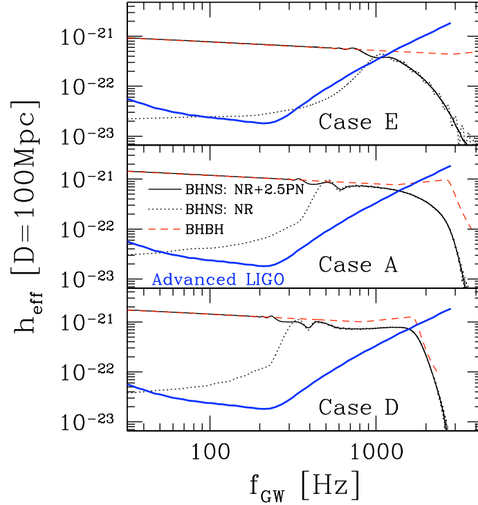
Figure 17.12: Gravitational wave power spectra for the q = 1, 3 and 5 cases (Cases E, A and D, respectively). The solid curve in each panel shows the combined waveform found by attaching the restricted 2.5 order PN waveform to the dominant modes computed by the numerical relativity simulation (NR), while the dotted curve shows the contribution from the latter only. The dashed curve shows the power spectrum for a nonspinning black hole binary merger (BHBH) for black holes with the same mass ratios as the black hole-neutron star binaries (BHNS); the later exhibit significantly less power at higher frequencies, due to tidal disruption. The heavier solid curve is the effective strain of the Advanced LIGO detector, defined by h_{\text{LIGO}}(f) (see text). To set physical units, we assume a neutron star rest mass of M_0 = 1.4M_\odot and a source distance of D=100\text{Mpc} . [From Etienne et al. (2009).]
