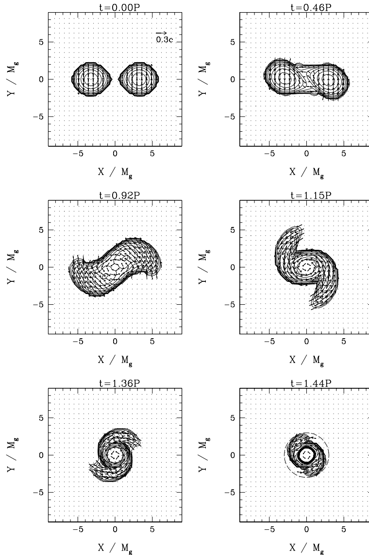
Figure 16.7: [CAMBRIDGE: replace M_g with M .] Same as Figure 16.5, but for a binary of total rest mass \bar{M}_0 = 0.332 (Model I3 in Table 16.1). Contour lines denote densities \rho_*/\rho_{*\max} = 10^{-0.3j} with \rho_{*\max} = 0.866 and j = 0, 1, 2, \dots, 10 . The dashed line in the last snapshot is the circle at r = 3M , which encloses over 99% of the total rest mass. The thick solid line at r/M \approx 1 denotes the location of the apparent horizon. [From Shibata and Uryū (2000).]
