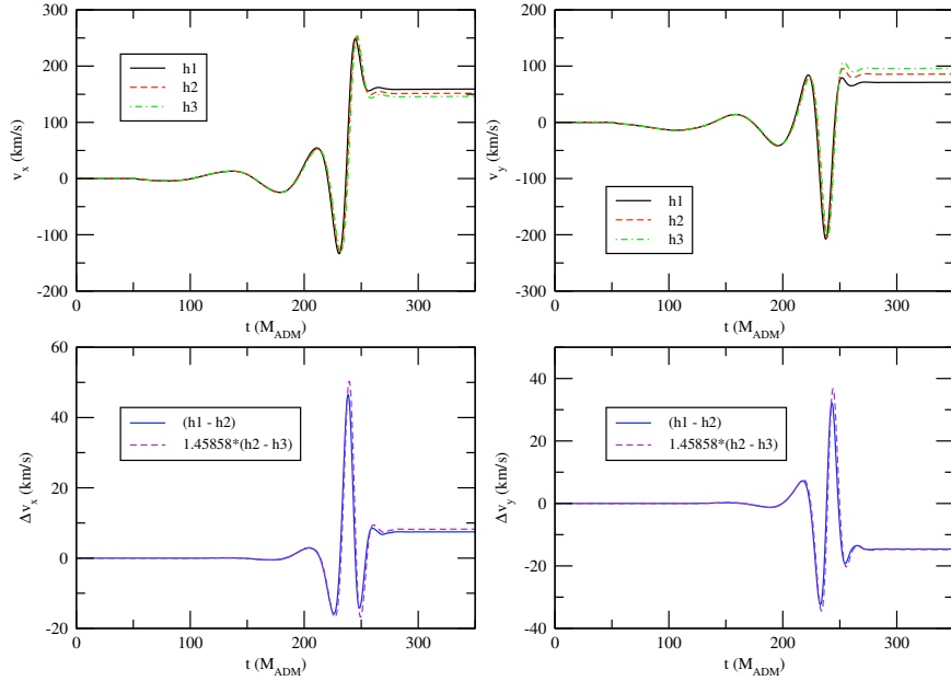
Figure 13.10: Components of the kick velocity as a function of time in the simulations of González et al. (2007) for a nonspinning binary of mass ratio q = 0.33 . The graphs shows results for three different resolutions, the finest of which are h_1 = m_1/45 , h_2 = m_1/51 , and h_3 = m_1/58 , where m_1 is the smaller black hole’s irreducible mass. The convergence test in the lower panels demonstrates second-order convergence. As expected, the kick velocity oscillates during the inspiral, and then remains constant once the emission of linear momentum ceases. [From González et al. (2007).]
