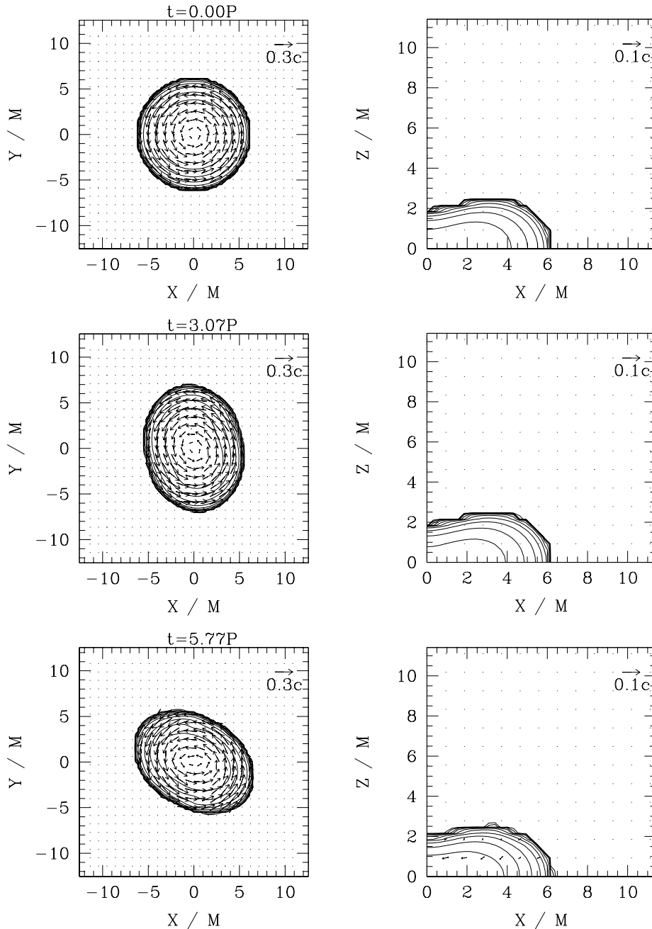
Figure 14.7: Snapshots of contours for the density \rho_* and the velocity field v^i in the equatorial plane (left) and in the meridional plane (right) for a bar-unstable model with R/M \approx 7.2 and \beta \approx 0.25 . The contour lines are drawn for \rho_*/\bar{\rho}_{* \max} = 10^{-0.3j} for j = 0, 1, 2, \dots, 10 where \bar{\rho}_{* \max} is 0.128, 0.152 and 0.176 at the three different times. The lengths of arrows are normalized to 0.3c (left) and 0.1c (right). The time is shown in units of the initial central period P \approx 15M . [From Shibata et al. (2000b).]
