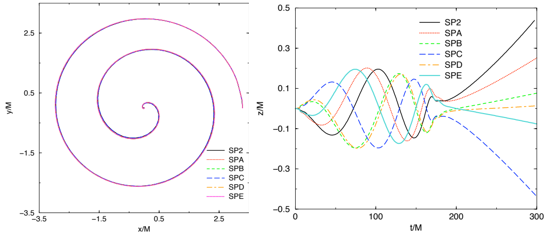
Figure 13.13: The left panel shows the projection into the x - y (orbital) plane of the puncture trajectories for six different sets of initial data (with only one puncture shown per binary). All binaries have equal masses and black hole spins of magnitude S/m^2 = 0.5 that reside in the orbital plane and are anti-aligned with each other; however, the direction of the spins within the orbital plane are different for each set of initial data. In this case the spin hardly affects the trajectory of the black holes within the x - y plane. The right panel shows the z -location of the orbital plane as a function of time. During the inspiral, the orbital plane oscillates along the z -axis, but does not tilt. Following merger, the remnant recoils along the z -axis. [From Campanelli et al. (2007b).]
