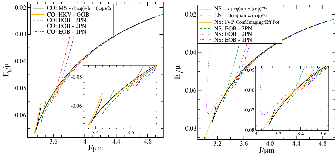
Figure 12.7: [CAMBRIDGE: replace m with M in label.] The equilibrium binding energy E_b versus the total equilibrium angular momentum J for the same corotational (left panel) and nonspinning (right panel) binaries shown in Figure 12.6. [From Cook and Pfeiffer (2004) and Caudill et al. (2006).]
