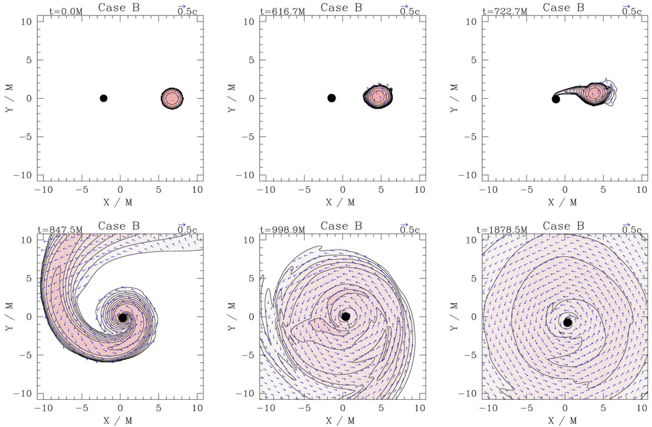
Figure 17.14: Snapshots of rest-density contours and 3-velocity vectors at selected times during the merger of an irrotational neutron star orbiting a black hole with spin a/M_{\text{BH}} = J_{\text{BH}}/M_{\text{BH}}^2 = 0.75 , as shown in Figure 17.13 (case B). The contours represent the density in the orbital plane, plotted according to \rho_0 = \rho_{0,\text{max}} 10^{-0.38j-0.04} , ( j=0, 1, \dots, 12 ), with darker grey scaling for higher density. The maximum initial neutron density is K\rho_{0,\text{max}} = 0.126 , where K is the initial polytropic gas constant, or \rho_{0,\text{max}} = 9 \times 10^{14} \text{g cm}^{-3} (1.4M_{\odot}/M_0)^2 . Arrows represent the velocity field in the orbital plane. The apparent horizon interior is marked by a filled black circle. In cgs units, the initial ADM mass for this case is M = 2.5 \times 10^{-5} (M_0/1.4M_{\odot}) s = 7.6 (M_0/1.4M_{\odot}) \text{km} . [From Etienne et al. (2009).]
