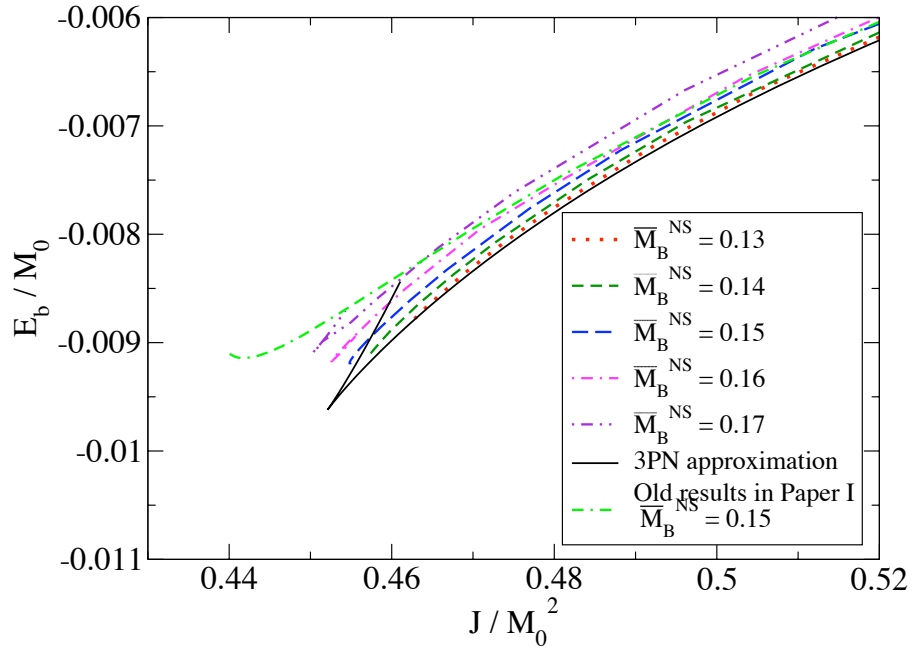
Figure 17.2: Binding energy E_b versus the total angular momentum J for a polytropic n = 1 binary with mass ratio q = 5 . The “old results in Paper I” refer to results obtained with the “leading-order spin approximation” for the parameter \Omega_{\text{spin}} in the black hole boundary conditions. The quantity \bar{M}^{\text{NS}} denotes the dimensionless (baryon) rest-mass of the neutron star and is larger for higher compactions; the maximum isolated mass corresponds to \bar{M}^{\text{NS}} = 0.18 [From Taniguchi et al. (2008).]
