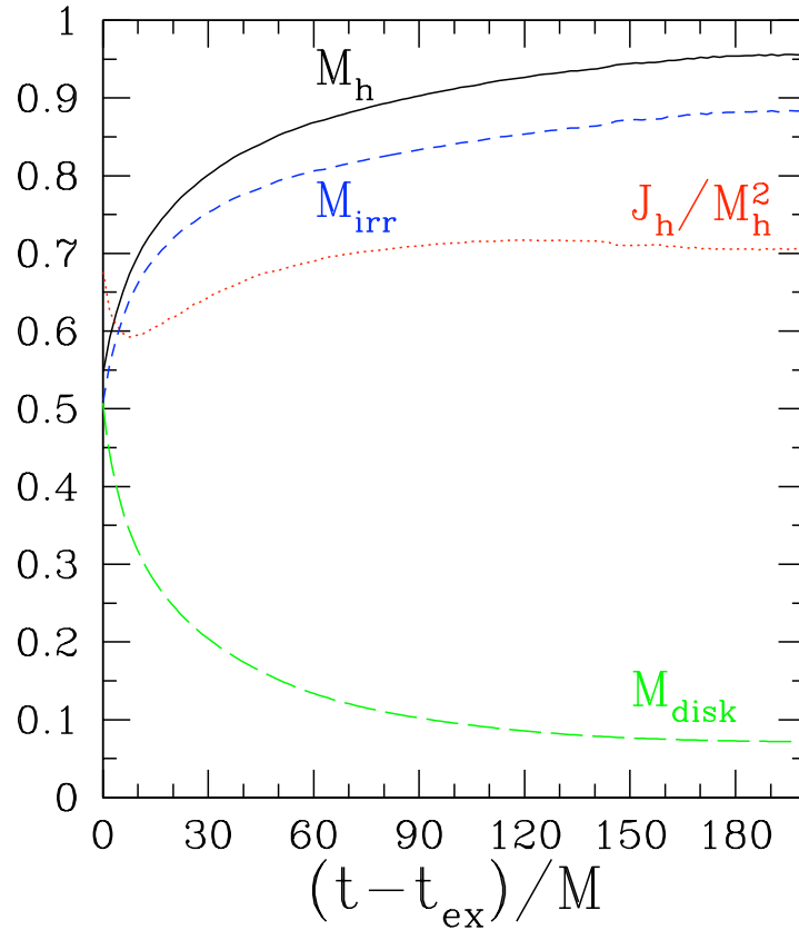
Figure 14.10: Post-excision evolution of the horizon mass M_h , spin parameter J_h/M_h^2 , and the irreducible mass M_{\text{irr}} of the central black hole, and the rest mass of the disk, M_{\text{disk}} , outside the apparent horizon. Time is measured from the beginning of excision ( t_{\text{ex}} = 28284M ) [From Liu et al. (2007).]
