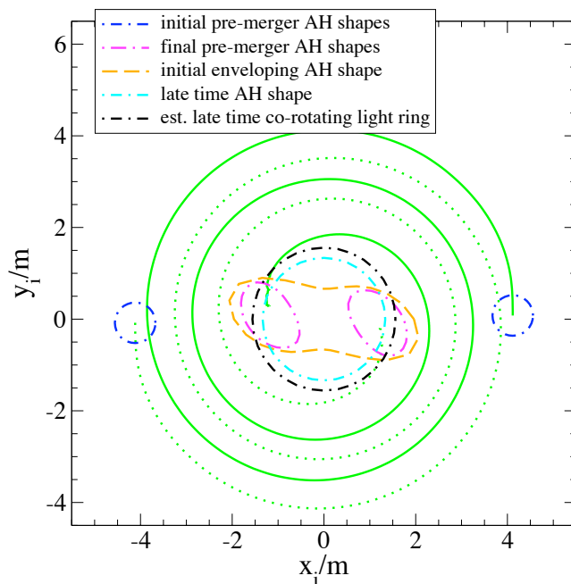
Figure 13.4: The evolution in the orbital plan of an equal-mass, nonspinning binary black hole, showing the coordinate locations of the apparent horizons (AH) at several key moments during the inspiral and merger. [From Buonanno et al. (2007)].
