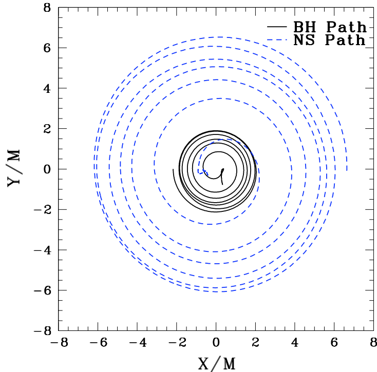
Figure 17.13: Trajectories of the black hole and neutron star coordinate centroids for the merger of an irrotational neutron star orbiting a spinning black hole with spin J_{\text{BH}}/M_{\text{BH}}^2 = 0.75 (case B). Compare with Figure 17.8 for the merger of an identical neutron star with a nonspinning black hole, assuming the same binary mass ratio q = 3 and initial orbital angular velocity M\Omega \approx 0.033 . [From Etienne et al. (2009).]
