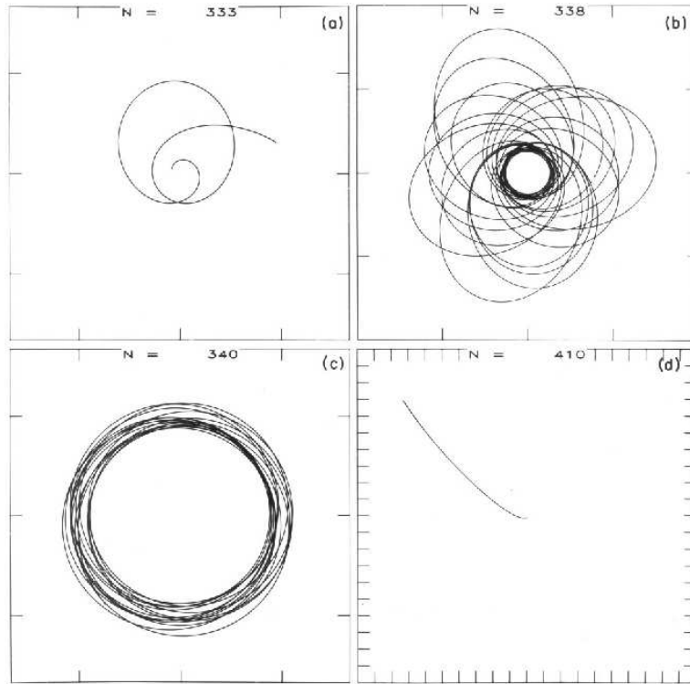
Figure 8.18: Orbital trajectories of four typical particles near the cluster center. Each particle N surrounds a fraction N/7198 of the total cluster rest mass at t = 0 . In each frame the spacing between radial grid marks is \Delta r_s = 1M . In (a) the particle is initially in an elliptical-like orbit, but spirals into the black hole after about two orbits. In (b) the particle moves in a nearly elliptical orbit, exhibiting large perihelion precession about the central hole. In (c) the particle moves essentially unperturbed in a nearly circular orbit. In (d) the particle falls nearly radially into the black hole. [From Shapiro and Teukolsky (1986)].
