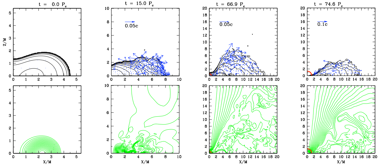
Figure 14.14: The upper 4 panels show snapshots of the rest-mass density contours and velocity vectors on the meridional plane. The lower panels show the field lines (lines of constant A_\phi ) for the poloidal magnetic field at the same times as the upper panels. The density contours are drawn for \rho^*/\rho_{\max,0}^* = 10^{-0.3i-0.09} ( i = 0-12 ). The field lines are drawn for A_\phi = A_{\phi,\min} + (A_{\phi,\max} - A_{\phi,\min})i/20 ( i = 1-19 ), where A_{\phi,\max} and A_{\phi,\min} are the maximum and minimum value of A_\phi respectively at the given time. The thick solid curves in the lower left corners denote the apparent horizon. [From Duez et al. (2006a).]
