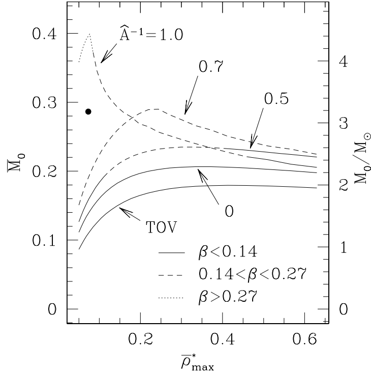
Figure 14.1: Maximum rest-mass configurations versus maximum mass-energy density for differentially rotating n = 1 sequences of constant \hat{A}^{-1} . Values of \beta = T/|W| for the models are indicated. The mass–density curve for static TOV equilibrium stars is shown for comparison. The supramassive limit for uniformly rotating stars corresponds to the curve \hat{A}^{-1} = 0 . Masses are given in nondimensional units on the left-hand side ( K = 1 ) and in solar masses on the right-hand side; the later are calculated by assigning the maximum rest-mass for nonrotating stars to 2 M_{\odot} . The dot marks one particular hypermassive configuration whose stability properties we will study below. [From Baumgarte et al. (2000).]
