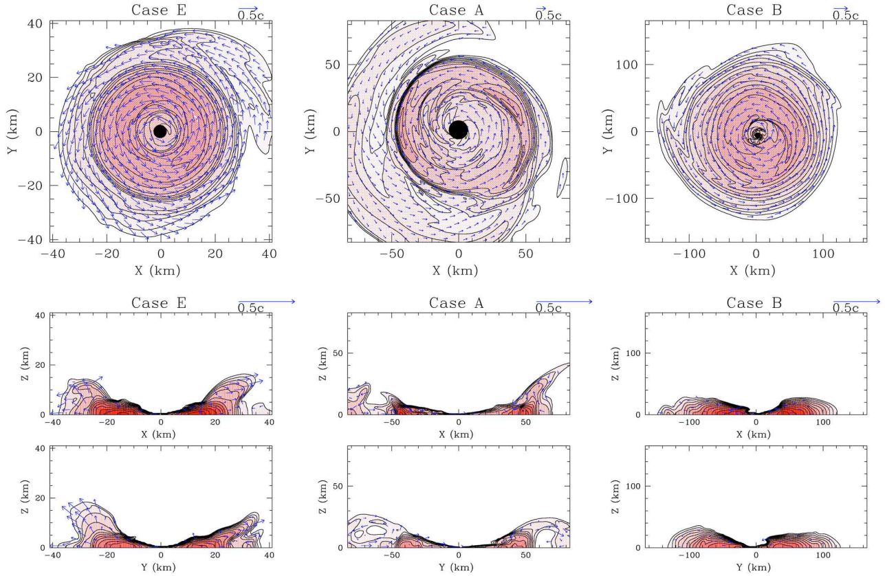
Figure 17.16: Snapshots of rest-density contours and 3-velocity vectors at the end of the simulations for three binary black hole-neutron star merger scenarios (see text). The remnant disks are shown in the orbital plane (upper row) and meridional plane (bottom rows). The contours represent the density plotted according to \rho_0 = \rho_{0,\max} 10^{-0.1j-3.3} ( j=0, 1, \dots, 13 ) for Cases A and B and \rho_0 = \rho_{0,\max} 10^{-0.19j-2.32} ( j=0, 1, \dots, 12 ) for Case E, with darker grey scaling for higher density. In all cases the maximum initial neutron density is K\rho_{0,\max} = 0.126 , where K is the initial polytropic gas constant, or \rho_{0,\max} = 9 \times 10^{14} \text{g cm}^{-3} (1.4M_\odot/M_0)^2 . Arrows represent the velocity field. The apparent horizon interior in the orbital plane is marked by a filled black circle. Length scales are specified in km, assuming the neutron star has a rest mass of 1.4M_\odot ; it can be converted to units of M via the formula M = 1.9(q+1)\text{km} . [After Etienne et al. (2009).]
