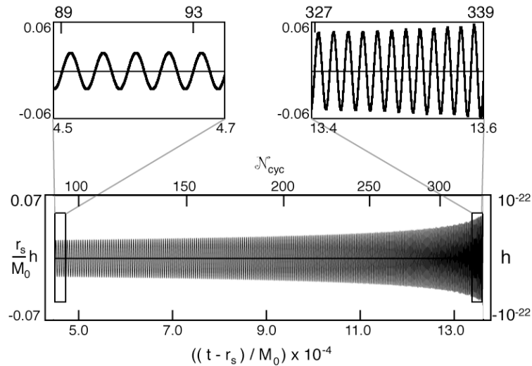
Figure 15.7: The final hundreds of cycles of the inspiral gravitational waveform measured along the axis of rotation by a distant observer as a function of retarded time and cycle number for an irrotational binary neutron star system. The numbers give the strain h for a binary of total rest mass M_0 = 2 \times 1.5M_\odot at a distance r_s = 100 Mpc. [From Duez et al. (2002).]
