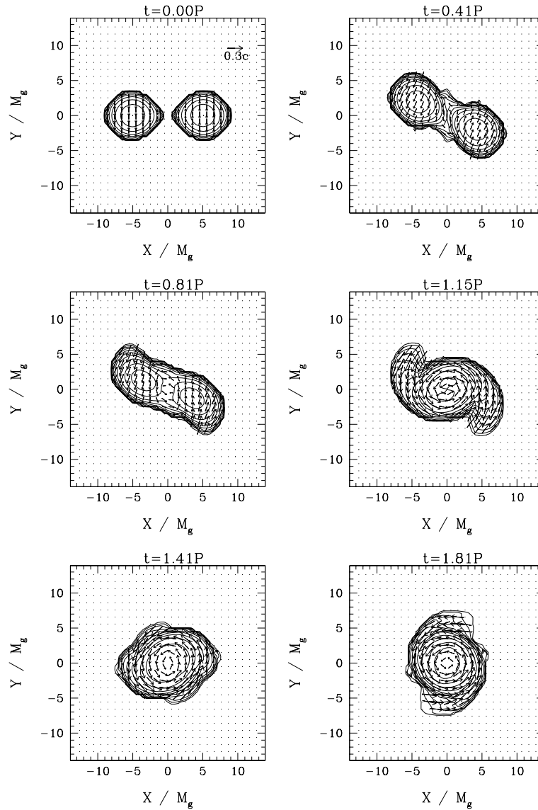
Figure 16.5: [CAMBRIDGE: Replace M_g with M . Then eliminate last sentence in this caption.] Snapshots of density contours for \rho_* = \gamma^{1/2}\rho_0 W (see equation 5.12) and the velocity field (v^x, v^y) in the equatorial plane for the coalescence of an irrotational binary of total rest mass \bar{M}_0 = 0.261 (Model I1 in Table 16.1). Time is measured in terms of the initial orbital period P . The contour lines denote densities \rho_*/\rho_{* \max} = 10^{-0.3j} with \rho_{* \max} = 0.255 and j = 0, 1, 2, \dots, 10 . The quantity M_g = M is the total initial ADM mass. [From Shibata and Uryū (2000).]
