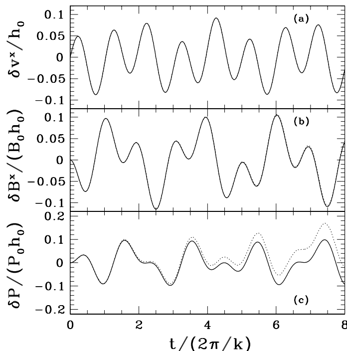
Figure 5.4: Analytic and numerical solutions for the perturbations of a magnetized fluid due to the presence of a linear, standing gravitational wave. The thick solid and thin dotted lines represent, respectively, the analytic and numerical solutions, though the two lines are not readily distinguishable in plots (a) and (b). All quantities are evaluated at z = 1/8 and are normalized as indicated. Time is normalized by the gravitational wave period. [From Duez et al. (2005b).]
