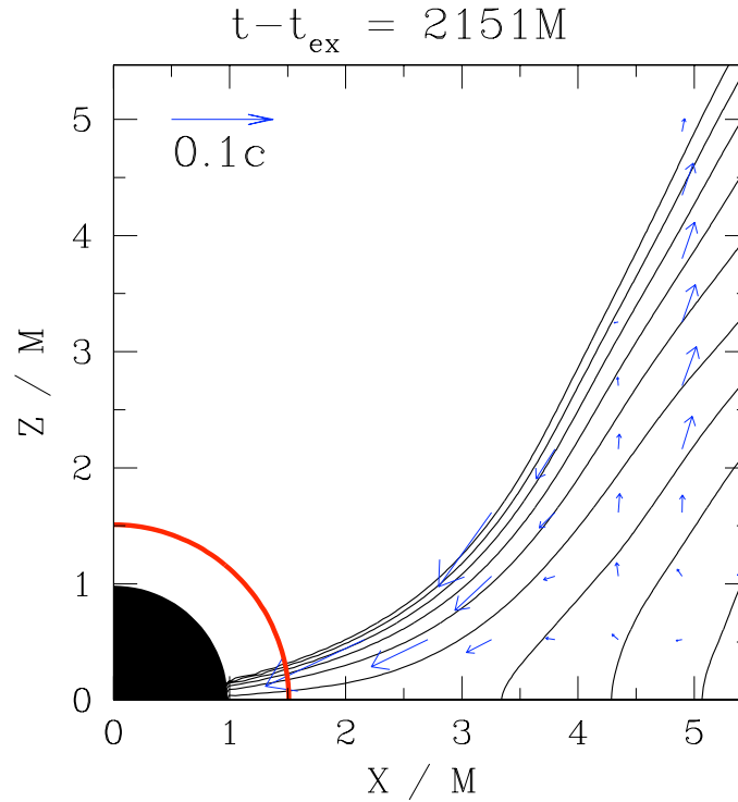
Figure 14.9: Blow-up of the meridional rest-mass density contours and velocity vectors at the end of the simulation, following excision and Cowling evolution. The density contours are drawn at for \rho_0 = 100\rho_{0c}(0)10^{-0.3j} ( j = 0-10 ). The thick solid (red) curve denotes the apparent horizon, and the dark region denotes the excision zone. [After Liu et al. (2007).]
