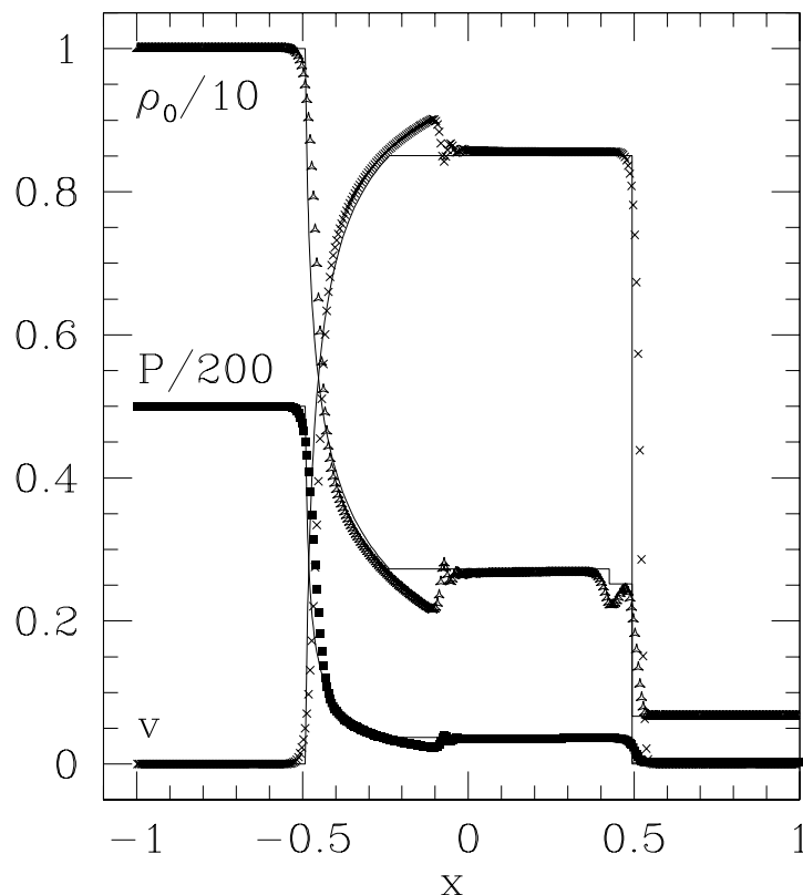
Figure 5.1: A one-dimensional relativistic Riemann shock tube test for an ideal fluid with an adiabatic index \Gamma = 2 . The plot shows the numerically evolved rest density \rho_0 (triangles), pressure P (squares), and velocity v (crosses) at t = 0.5 . The analytic values are indicated by solid curves. This calculation used the Wilson scheme with artificial viscosity P_{\text{vis}} = C_{\text{vis}} A (\delta v)^2 , A = \gamma^{1/2} \epsilon D , \delta v = 2 \partial_k v^k \Delta x and C_{\text{vis}} = 1 . [From Duez et al. (2003).]
